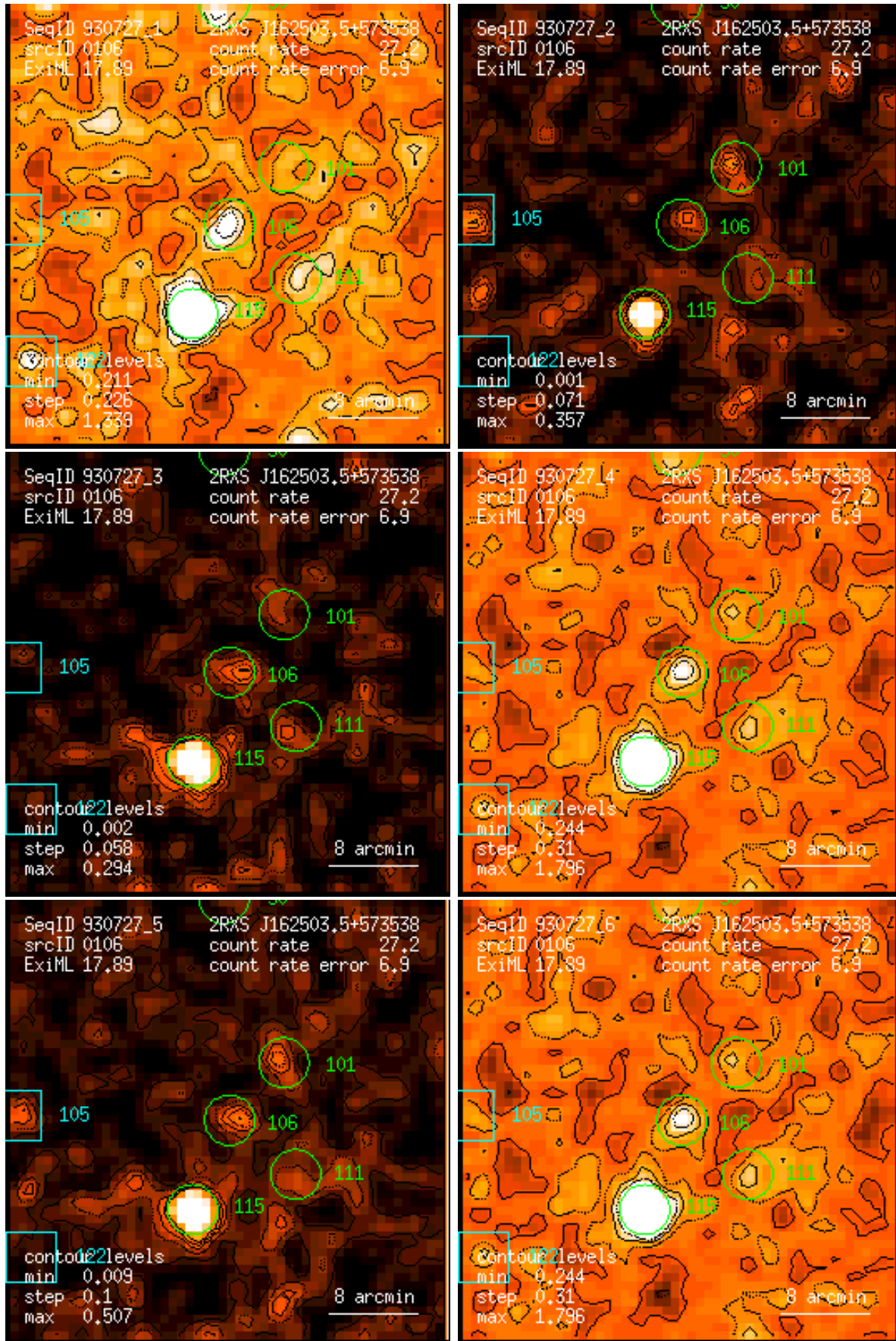
Figure 106: RASS 930727: detection 0106: band rate images, Gaussian filter: (1) PSPC channels 11 – 41, (2) 52 – 90, (3) 91 – 201, (4) 11 – 235, (5) 52 – 201, (6) 11 – 201. Broad band rates in counts/ks. Band rate contour levels in counts/ks/arcmin 2 .
