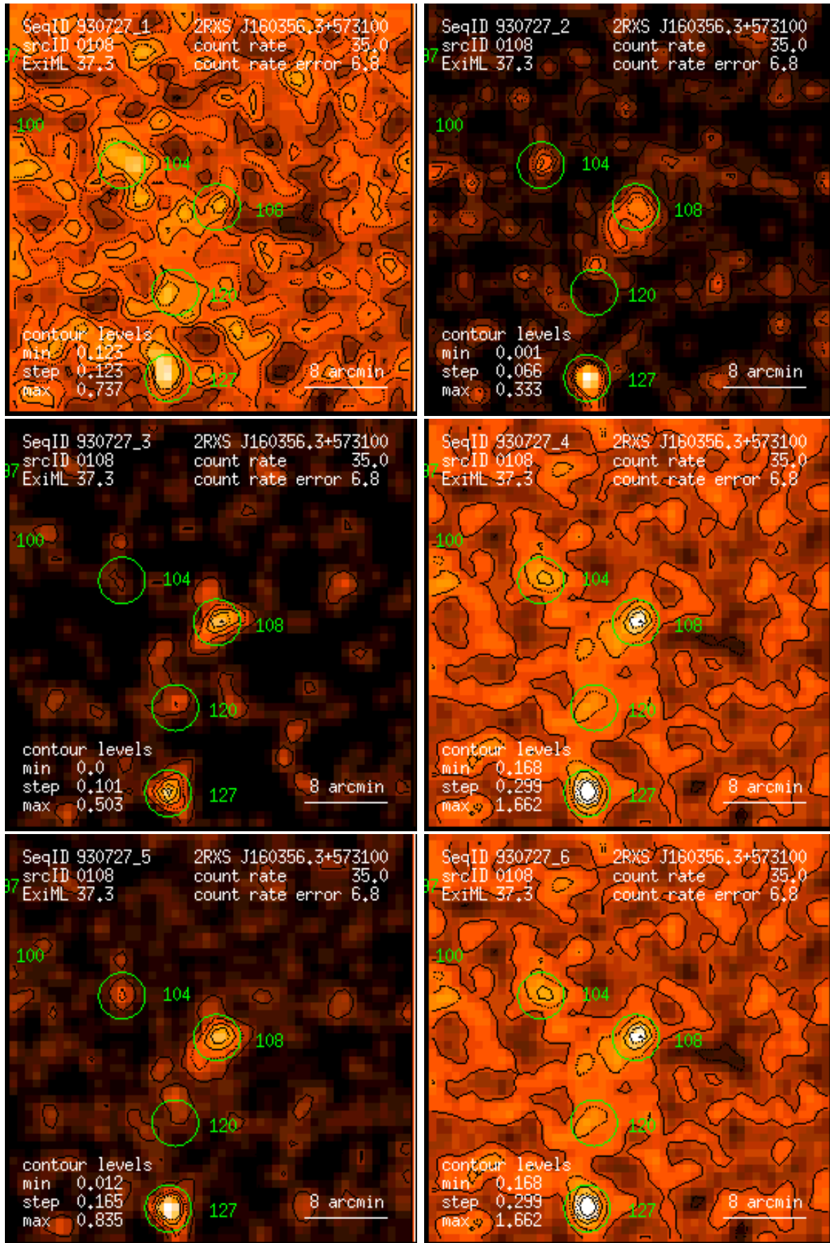
Figure 108: RASS 930727: detection 0108: band rate images, Gaussian filter: (1) PSPC channels 11 – 41, (2) 52 – 90, (3) 91 – 201, (4) 11 – 235, (5) 52 – 201, (6) 11 – 201. Broad band rates in counts/ks. Band rate contour levels in counts/ks/arcmin 2 .
