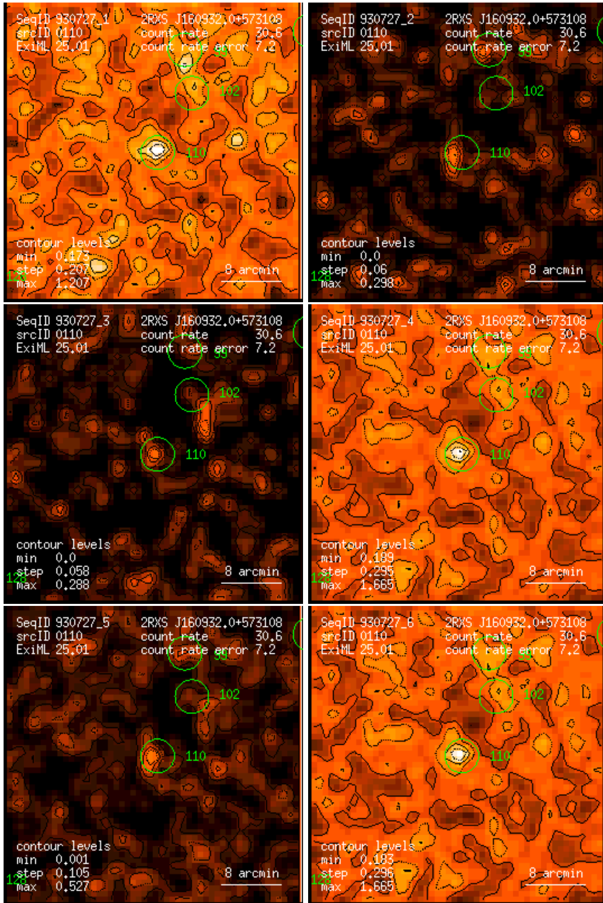
Figure 110: RASS 930727: detection 0110: band rate images, Gaussian filter: (1) PSPC channels 11 – 41, (2) 52 – 90, (3) 91 – 201, (4) 11 – 235, (5) 52 – 201, (6) 11 – 201. Broad band rates in counts/ks. Band rate contour levels in counts/ks/arcmin 2 .
