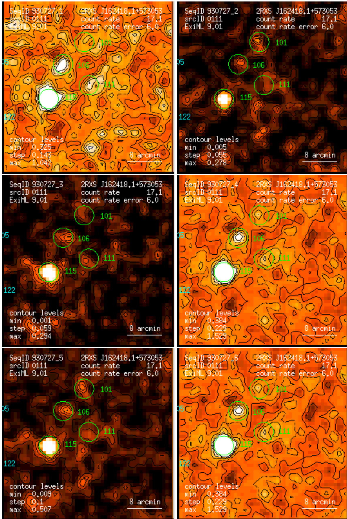
Figure 111: RASS 930727: detection 0111: band rate images, Gaussian filter: (1) PSPC channels 11 – 41, (2) 52 – 90, (3) 91 – 201, (4) 11 – 235, (5) 52 – 201, (6) 11 – 201. Broad band rates in counts/ks. Band rate contour levels in counts/ks/arcmin 2 .
