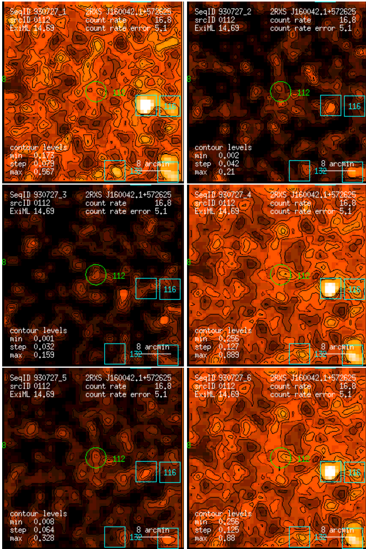
Figure 112: RASS 930727: detection 0112: band rate images, Gaussian filter: (1) PSPC channels 11 – 41, (2) 52 – 90, (3) 91 – 201, (4) 11 – 235, (5) 52 – 201, (6) 11 – 201. Broad band rates in counts/ks. Band rate contour levels in counts/ks/arcmin 2 .
