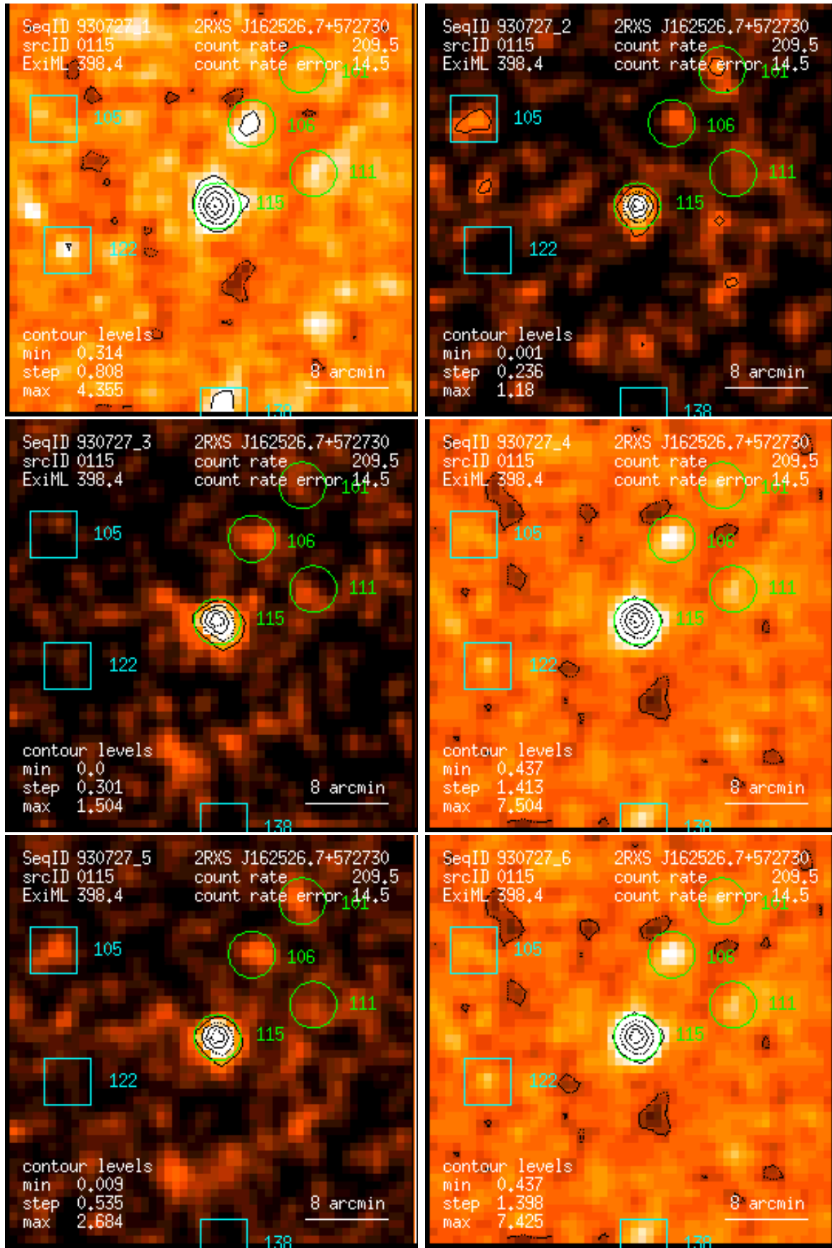
Figure 115: RASS 930727: detection 0115: band rate images, Gaussian filter: (1) PSPC channels 11 – 41, (2) 52 – 90, (3) 91 – 201, (4) 11 – 235, (5) 52 – 201, (6) 11 – 201. Broad band rates in counts/ks. Band rate contour levels in counts/ks/arcmin 2 .
