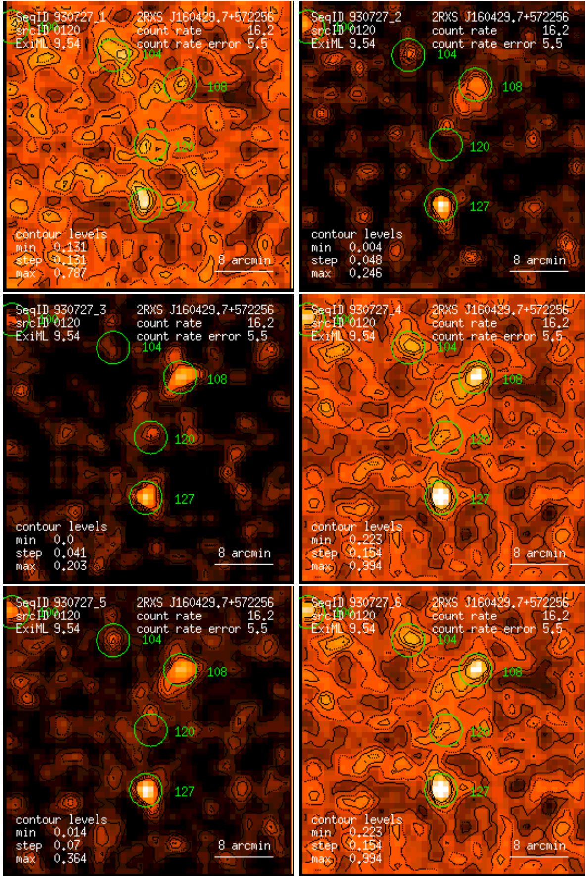
Figure 120: RASS 930727: detection 0120: band rate images, Gaussian filter: (1) PSPC channels 11 – 41, (2) 52 – 90, (3) 91 – 201, (4) 11 – 235, (5) 52 – 201, (6) 11 – 201. Broad band rates in counts/ks. Band rate contour levels in counts/ks/arcmin 2 .
