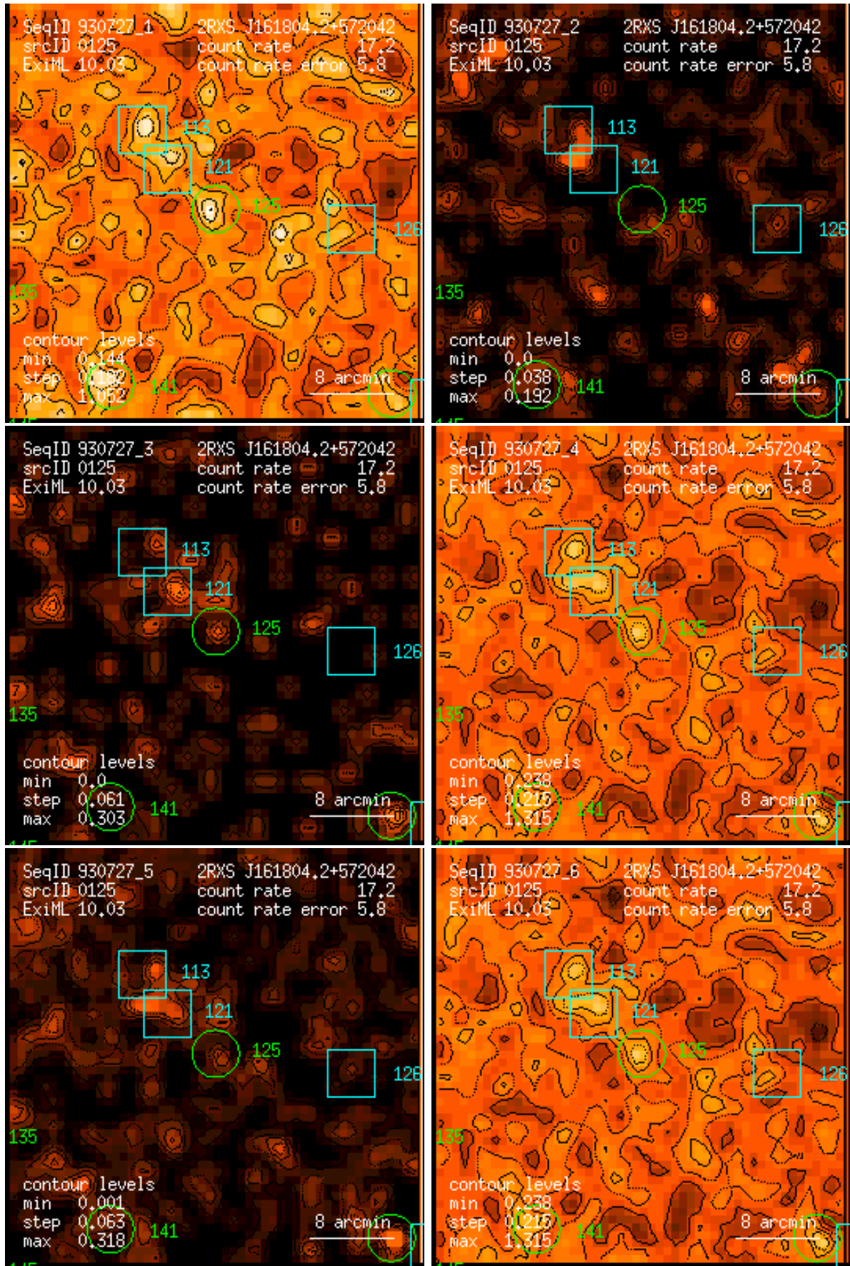
Figure 125: RASS 930727: detection 0125: band rate images, Gaussian filter: (1) PSPC channels 11 – 41, (2) 52 – 90, (3) 91 – 201, (4) 11 – 235, (5) 52 – 201, (6) 11 – 201. Broad band rates in counts/ks. Band rate contour levels in counts/ks/arcmin 2 .
