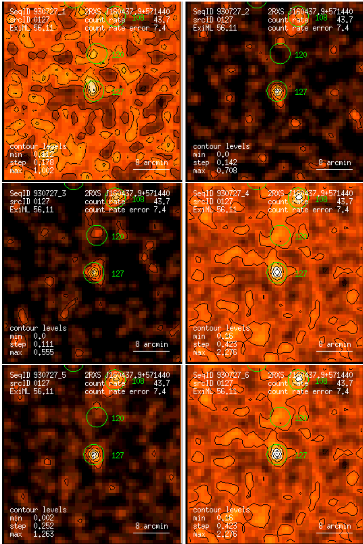
Figure 127: RASS 930727: detection 0127: band rate images, Gaussian filter: (1) PSPC channels 11 – 41, (2) 52 – 90, (3) 91 – 201, (4) 11 – 235, (5) 52 – 201, (6) 11 – 201. Broad band rates in counts/ks. Band rate contour levels in counts/ks/arcmin 2 .
