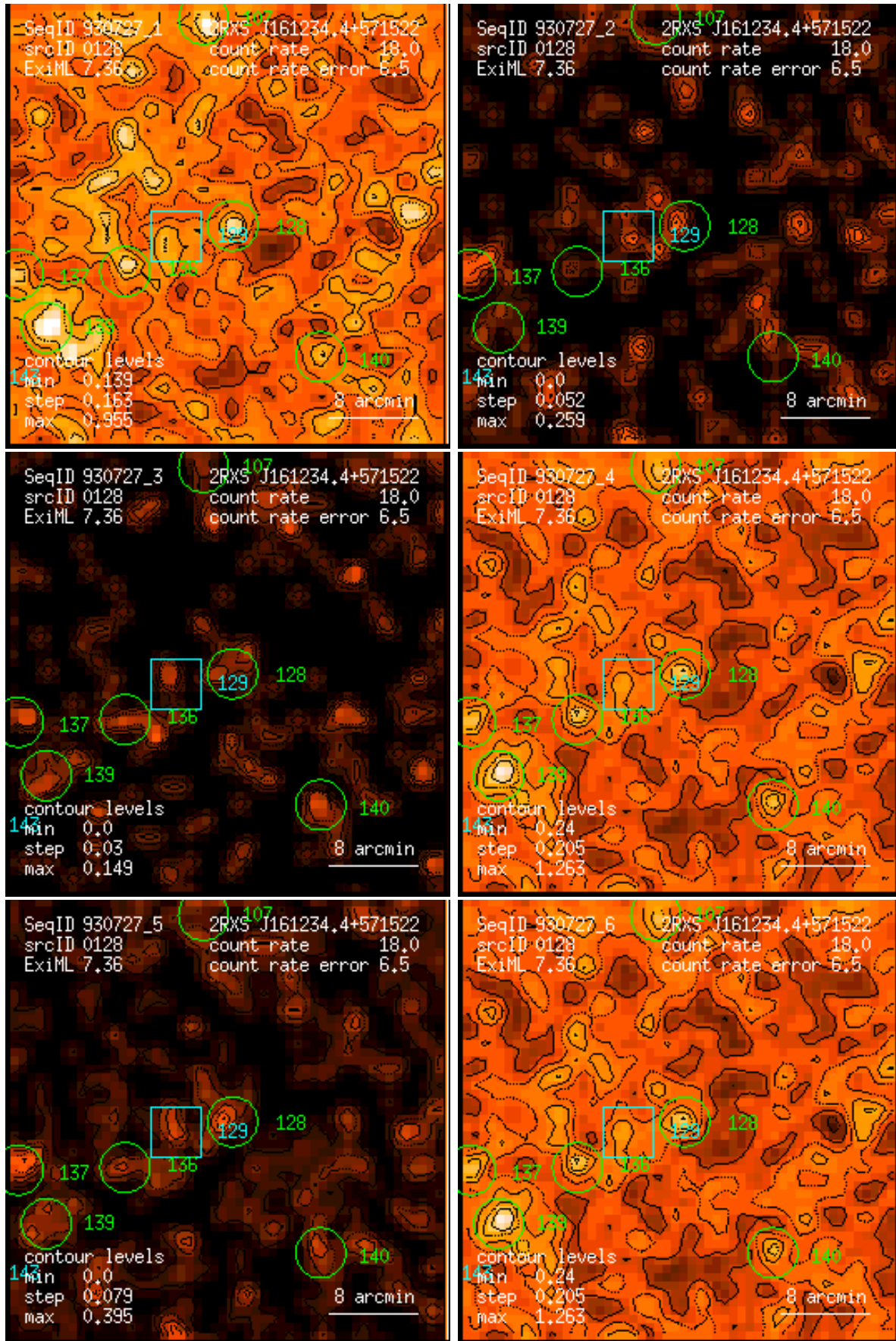
Figure 128: RASS 930727: detection 0128: band rate images, Gaussian filter: (1) PSPC channels 11 – 41, (2) 52 – 90, (3) 91 – 201, (4) 11 – 235, (5) 52 – 201, (6) 11 – 201. Broad band rates in counts/ks. Band rate contour levels in counts/ks/arcmin 2 .
