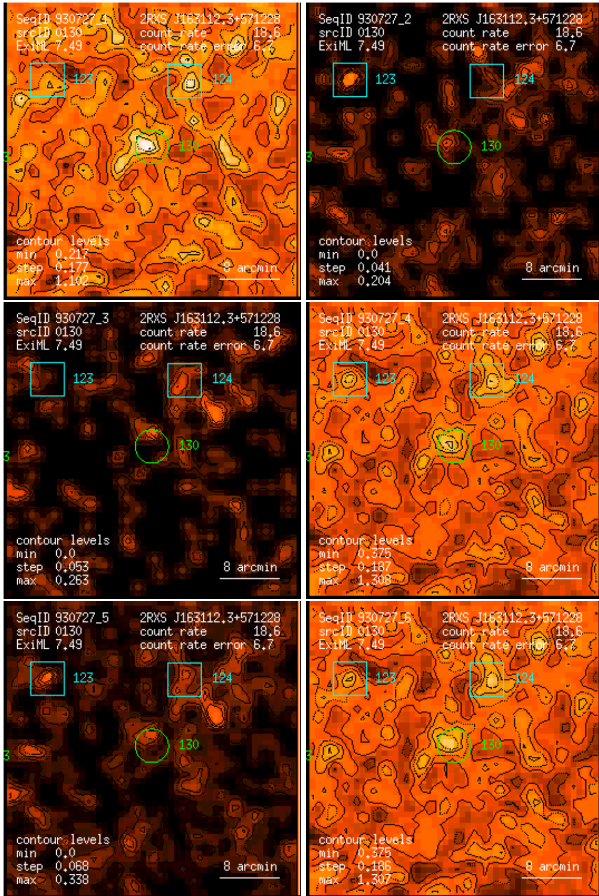
Figure 130: RASS 930727: detection 0130: band rate images, Gaussian filter: (1) PSPC channels 11 – 41, (2) 52 – 90, (3) 91 – 201, (4) 11 – 235, (5) 52 – 201, (6) 11 – 201. Broad band rates in counts/ks. Band rate contour levels in counts/ks/arcmin 2 .
