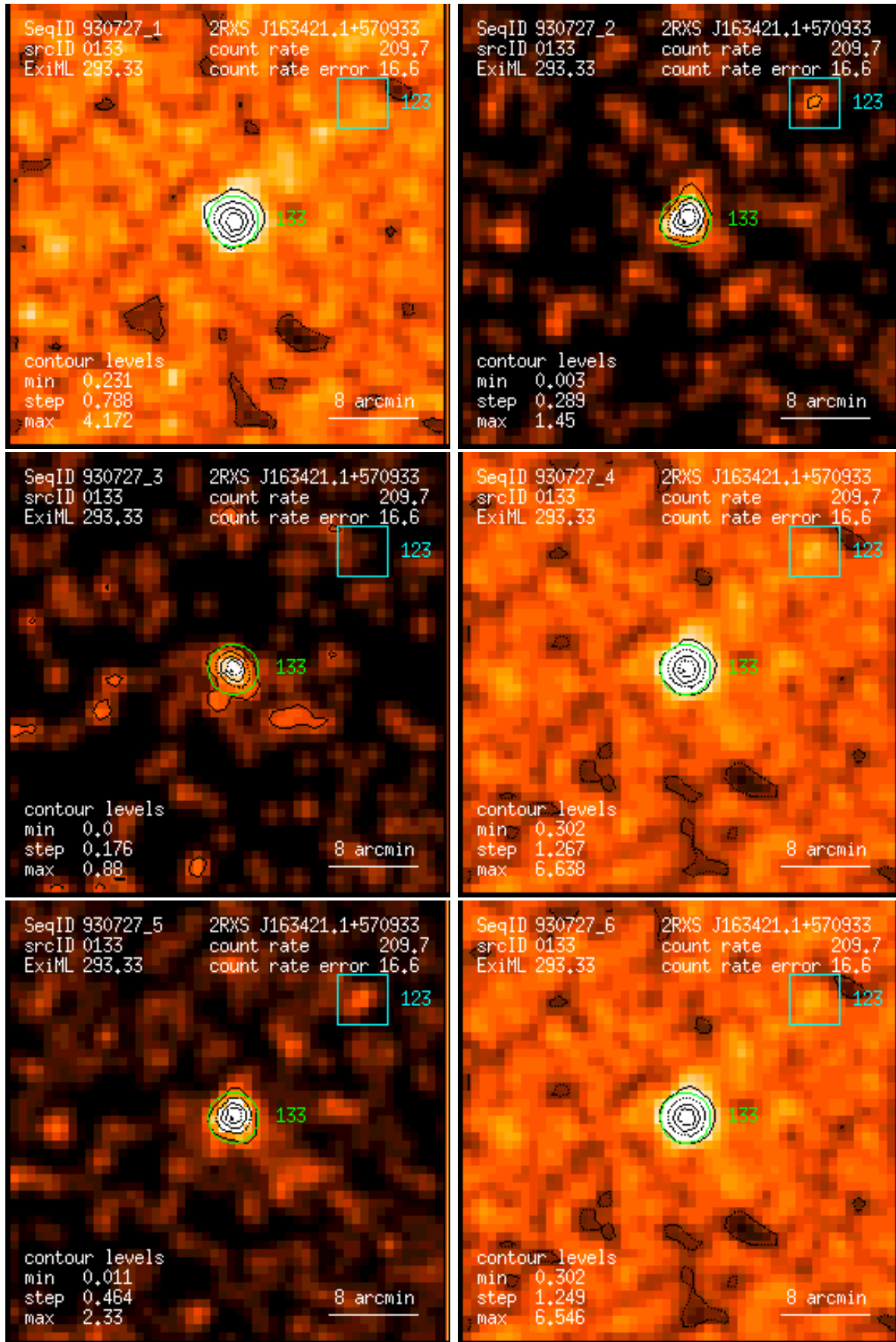
Figure 133: RASS 930727: detection 0133: band rate images, Gaussian filter: (1) PSPC channels 11 – 41, (2) 52 – 90, (3) 91 – 201, (4) 11 – 235, (5) 52 – 201, (6) 11 – 201. Broad band rates in counts/ks. Band rate contour levels in counts/ks/arcmin 2 .
