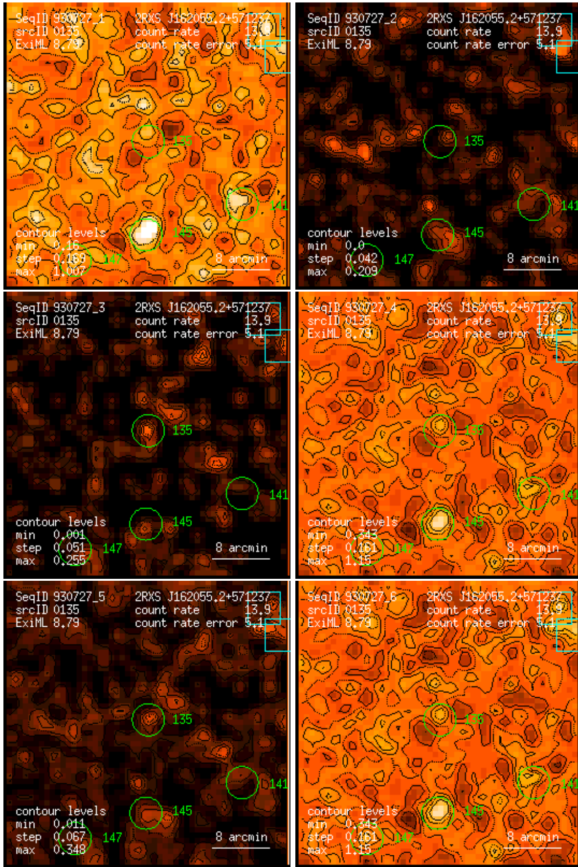
Figure 135: RASS 930727: detection 0135: band rate images, Gaussian filter: (1) PSPC channels 11 – 41, (2) 52 – 90, (3) 91 – 201, (4) 11 – 235, (5) 52 – 201, (6) 11 – 201. Broad band rates in counts/ks. Band rate contour levels in counts/ks/arcmin 2 .
