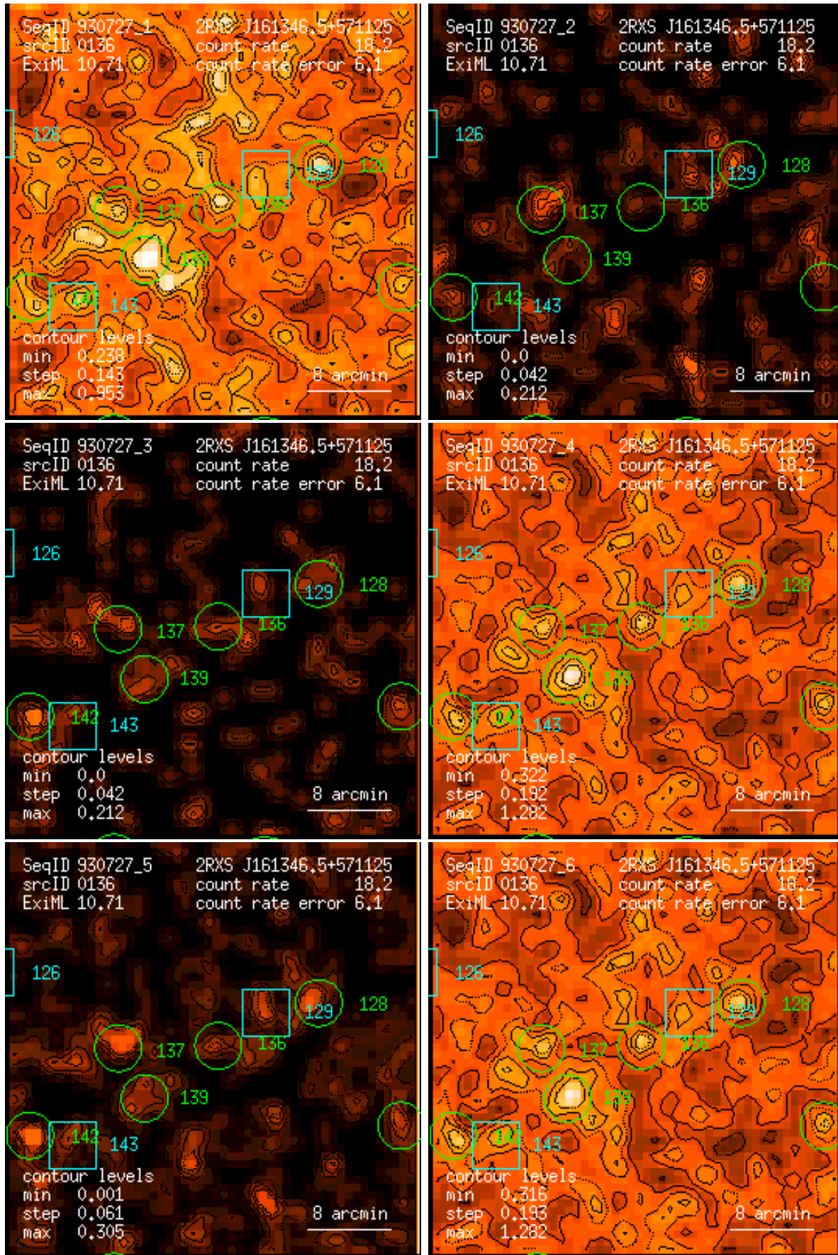
Figure 136: RASS 930727: detection 0136: band rate images, Gaussian filter: (1) PSPC channels 11 – 41, (2) 52 – 90, (3) 91 – 201, (4) 11 – 235, (5) 52 – 201, (6) 11 – 201. Broad band rates in counts/ks. Band rate contour levels in counts/ks/arcmin 2 .
