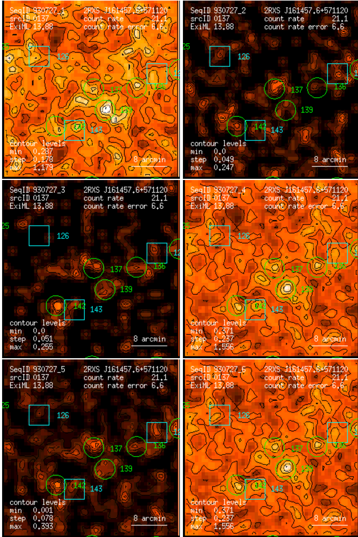
Figure 137: RASS 930727: detection 0137: band rate images, Gaussian filter: (1) PSPC channels 11 – 41, (2) 52 – 90, (3) 91 – 201, (4) 11 – 235, (5) 52 – 201, (6) 11 – 201. Broad band rates in counts/ks. Band rate contour levels in counts/ks/arcmin 2 .
