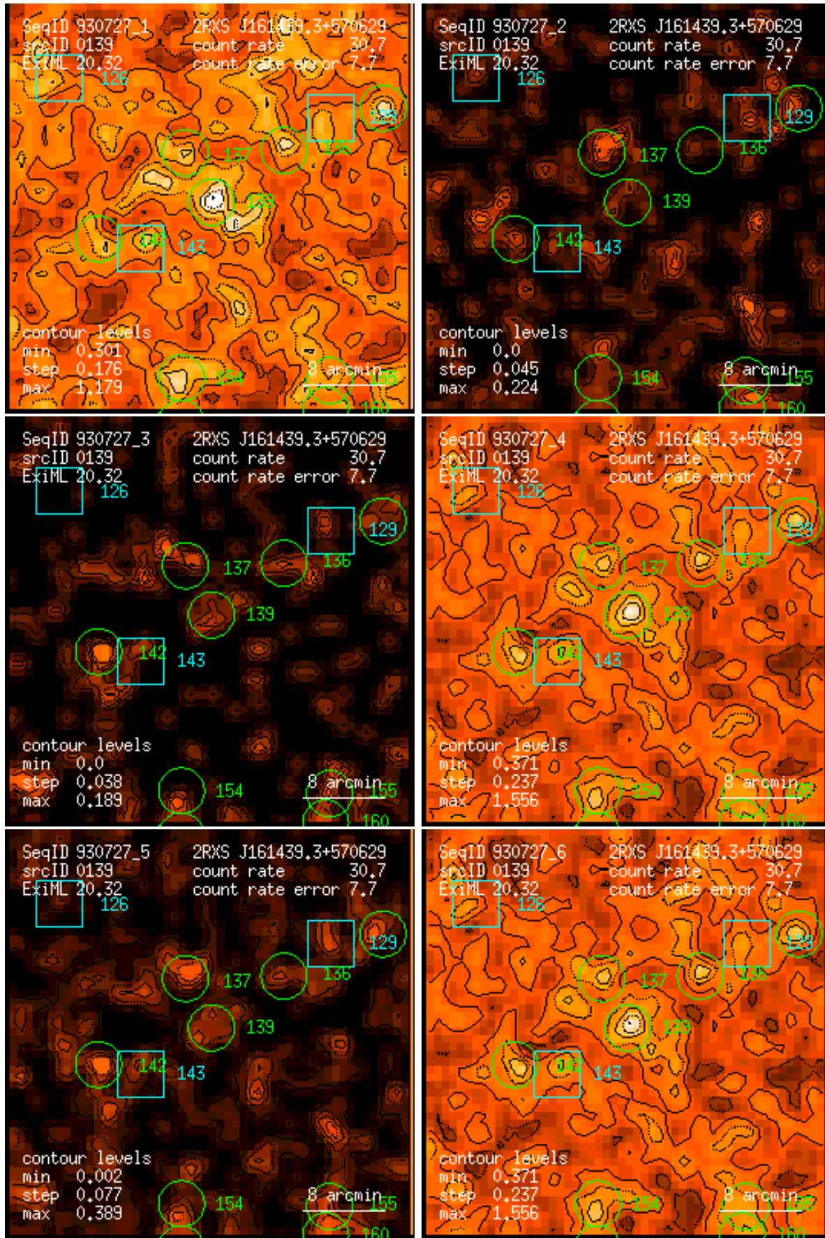
Figure 139: RASS 930727: detection 0139: band rate images, Gaussian filter: (1) PSPC channels 11 – 41, (2) 52 – 90, (3) 91 – 201, (4) 11 – 235, (5) 52 – 201, (6) 11 – 201. Broad band rates in counts/ks. Band rate contour levels in counts/ks/arcmin 2 .
