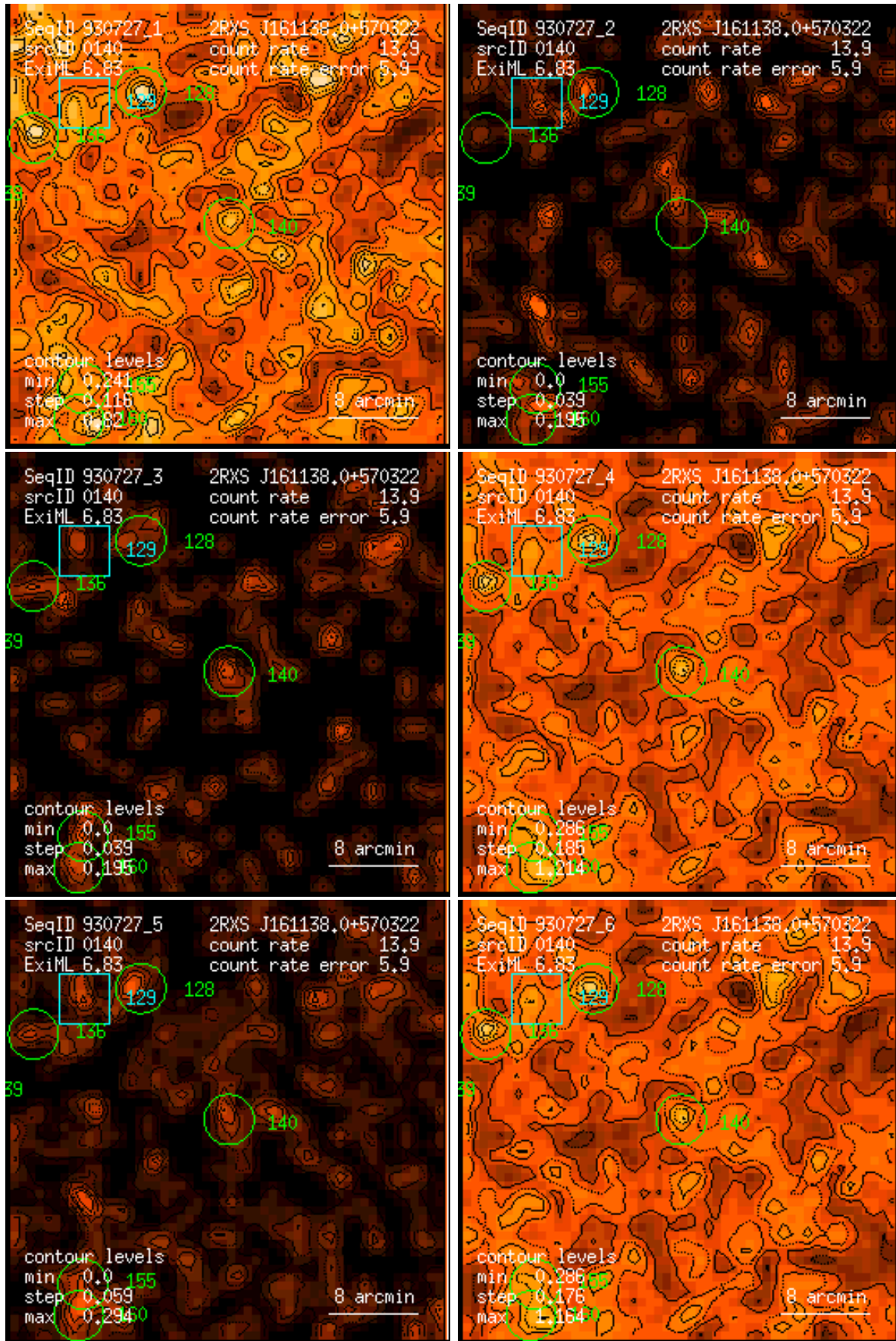
Figure 140: RASS 930727: detection 0140: band rate images, Gaussian filter: (1) PSPC channels 11 – 41, (2) 52 – 90, (3) 91 – 201, (4) 11 – 235, (5) 52 – 201, (6) 11 – 201. Broad band rates in counts/ks. Band rate contour levels in counts/ks/arcmin 2 .
