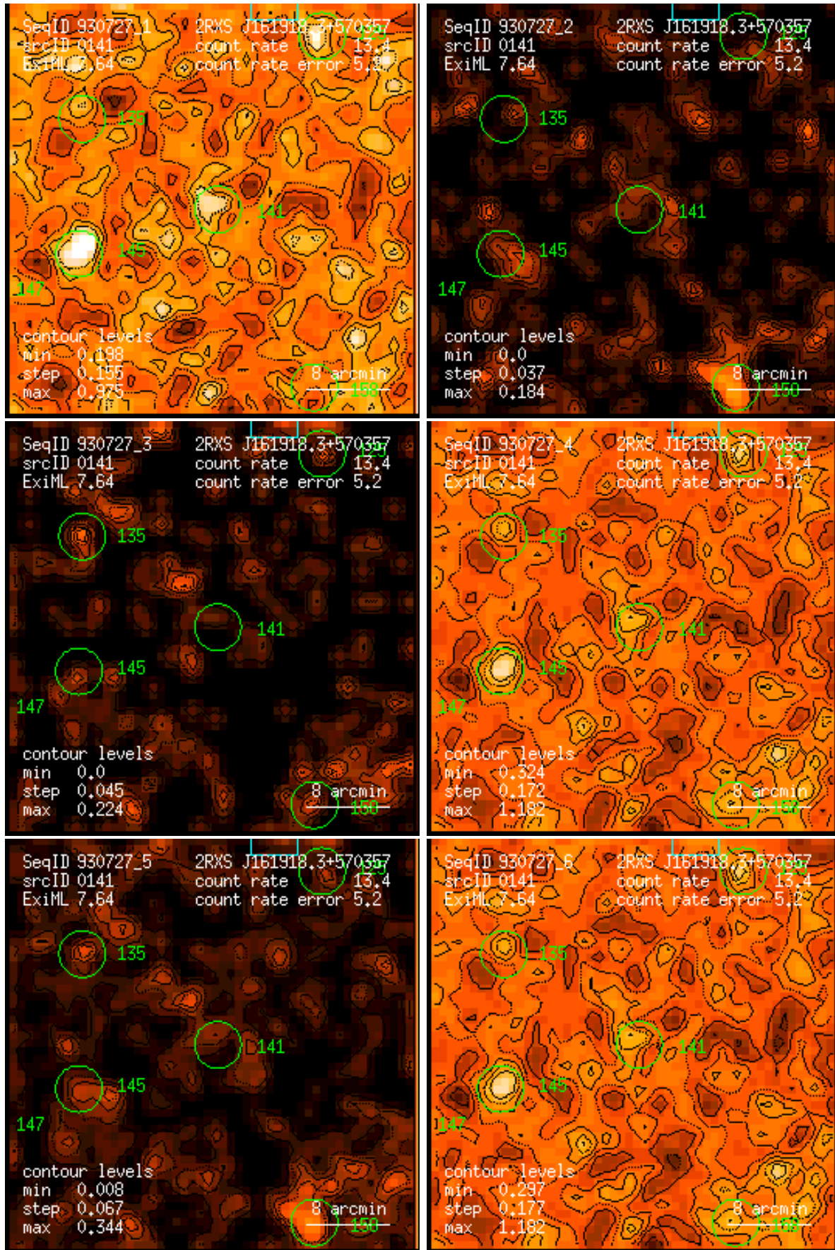
Figure 141: RASS 930727: detection 0141: band rate images, Gaussian filter: (1) PSPC channels 11 – 41, (2) 52 – 90, (3) 91 – 201, (4) 11 – 235, (5) 52 – 201, (6) 11 – 201. Broad band rates in counts/ks. Band rate contour levels in counts/ks/arcmin 2 .
