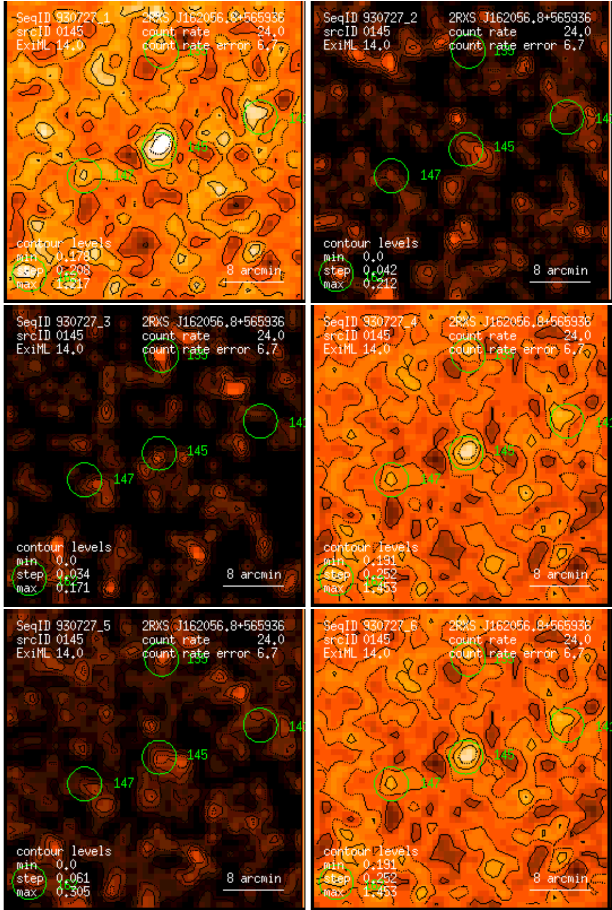
Figure 145: RASS 930727: detection 0145: band rate images, Gaussian filter: (1) PSPC channels 11 – 41, (2) 52 – 90, (3) 91 – 201, (4) 11 – 235, (5) 52 – 201, (6) 11 – 201. Broad band rates in counts/ks. Band rate contour levels in counts/ks/arcmin 2 .
