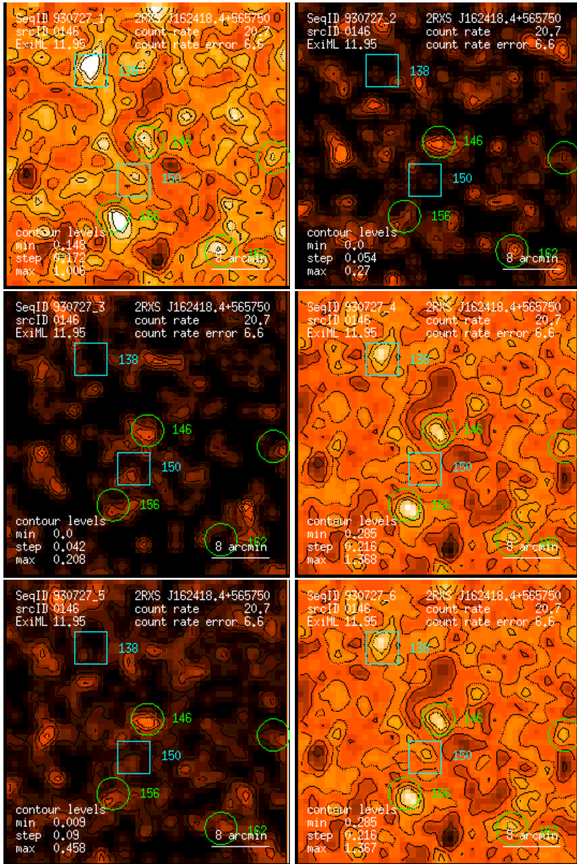
Figure 146: RASS 930727: detection 0146: band rate images, Gaussian filter: (1) PSPC channels 11 – 41, (2) 52 – 90, (3) 91 – 201, (4) 11 – 235, (5) 52 – 201, (6) 11 – 201. Broad band rates in counts/ks. Band rate contour levels in counts/ks/arcmin 2 .
