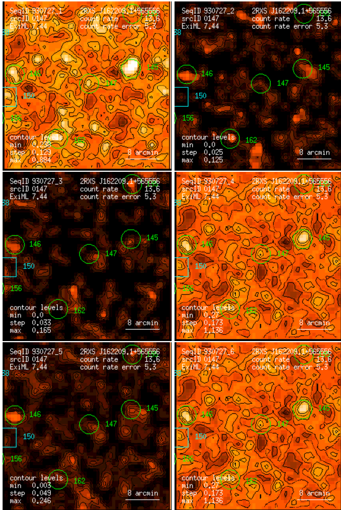
Figure 147: RASS 930727: detection 0147: band rate images, Gaussian filter: (1) PSPC channels 11 – 41, (2) 52 – 90, (3) 91 – 201, (4) 11 – 235, (5) 52 – 201, (6) 11 – 201. Broad band rates in counts/ks. Band rate contour levels in counts/ks/arcmin 2 .
