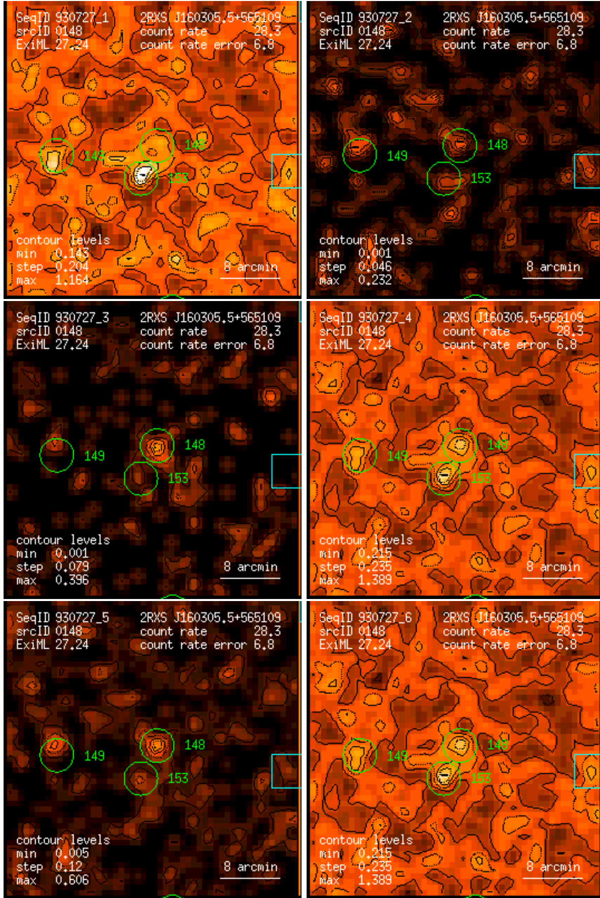
Figure 148: RASS 930727: detection 0148: band rate images, Gaussian filter: (1) PSPC channels 11 – 41, (2) 52 – 90, (3) 91 – 201, (4) 11 – 235, (5) 52 – 201, (6) 11 – 201. Broad band rates in counts/ks. Band rate contour levels in counts/ks/arcmin 2 .
