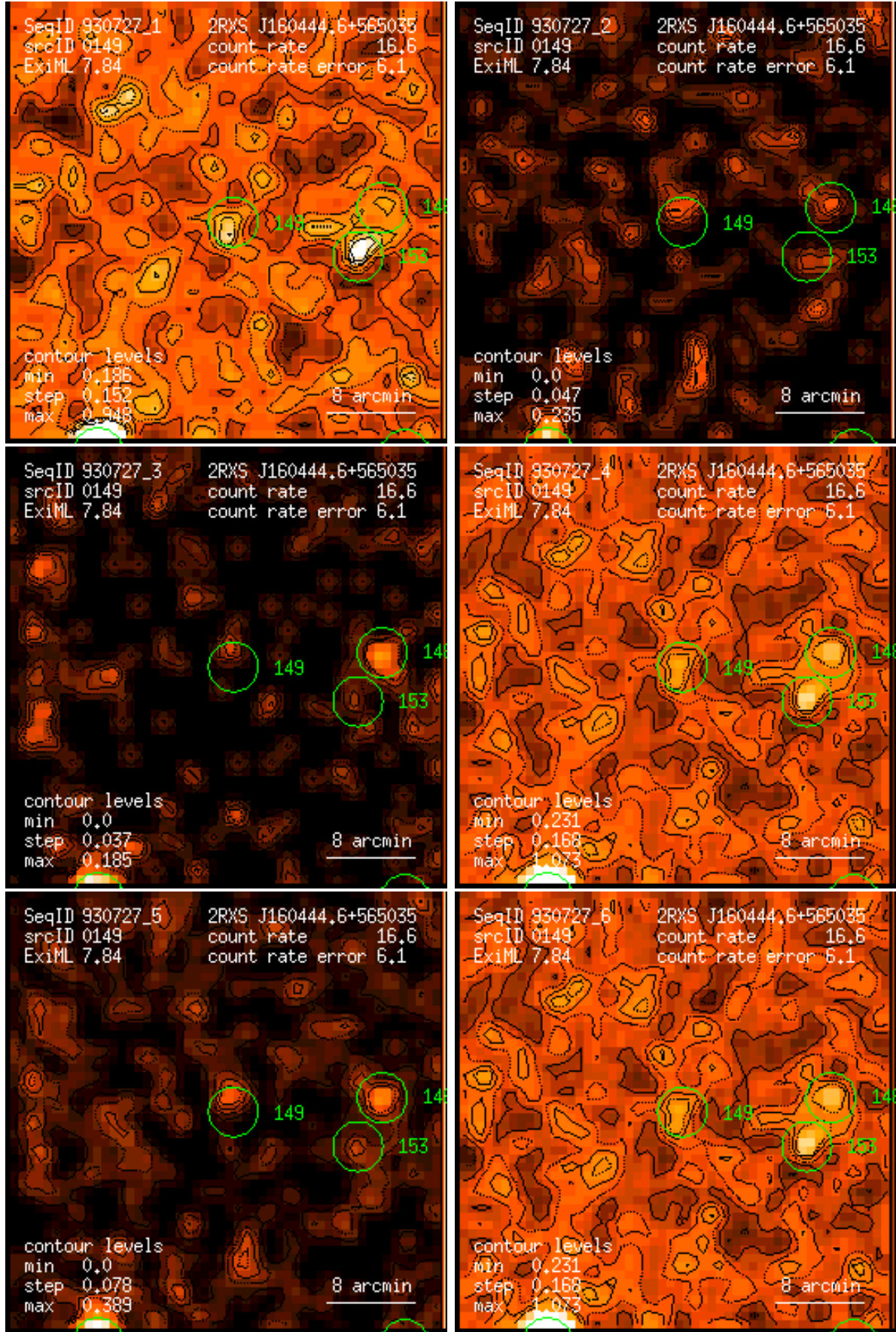
Figure 149: RASS 930727: detection 0149: band rate images, Gaussian filter: (1) PSPC channels 11 – 41, (2) 52 – 90, (3) 91 – 201, (4) 11 – 235, (5) 52 – 201, (6) 11 – 201. Broad band rates in counts/ks. Band rate contour levels in counts/ks/arcmin 2 .
