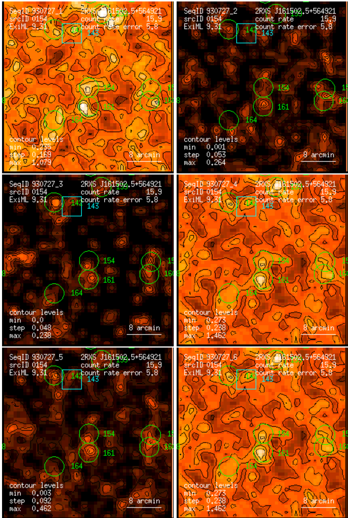
Figure 154: RASS 930727: detection 0154: band rate images, Gaussian filter: (1) PSPC channels 11 – 41, (2) 52 – 90, (3) 91 – 201, (4) 11 – 235, (5) 52 – 201, (6) 11 – 201. Broad band rates in counts/ks. Band rate contour levels in counts/ks/arcmin 2 .
