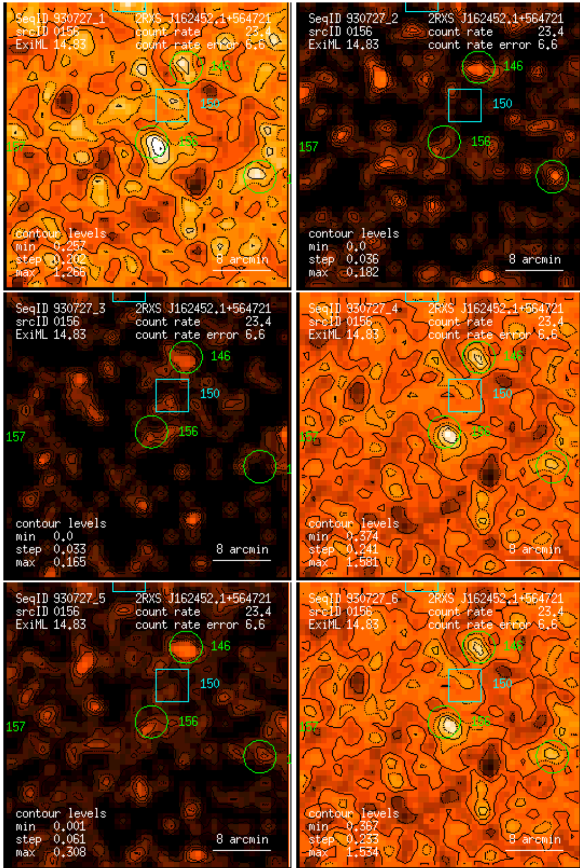
Figure 156: RASS 930727: detection 0156: band rate images, Gaussian filter: (1) PSPC channels 11 – 41, (2) 52 – 90, (3) 91 – 201, (4) 11 – 235, (5) 52 – 201, (6) 11 – 201. Broad band rates in counts/ks. Band rate contour levels in counts/ks/arcmin 2 .
