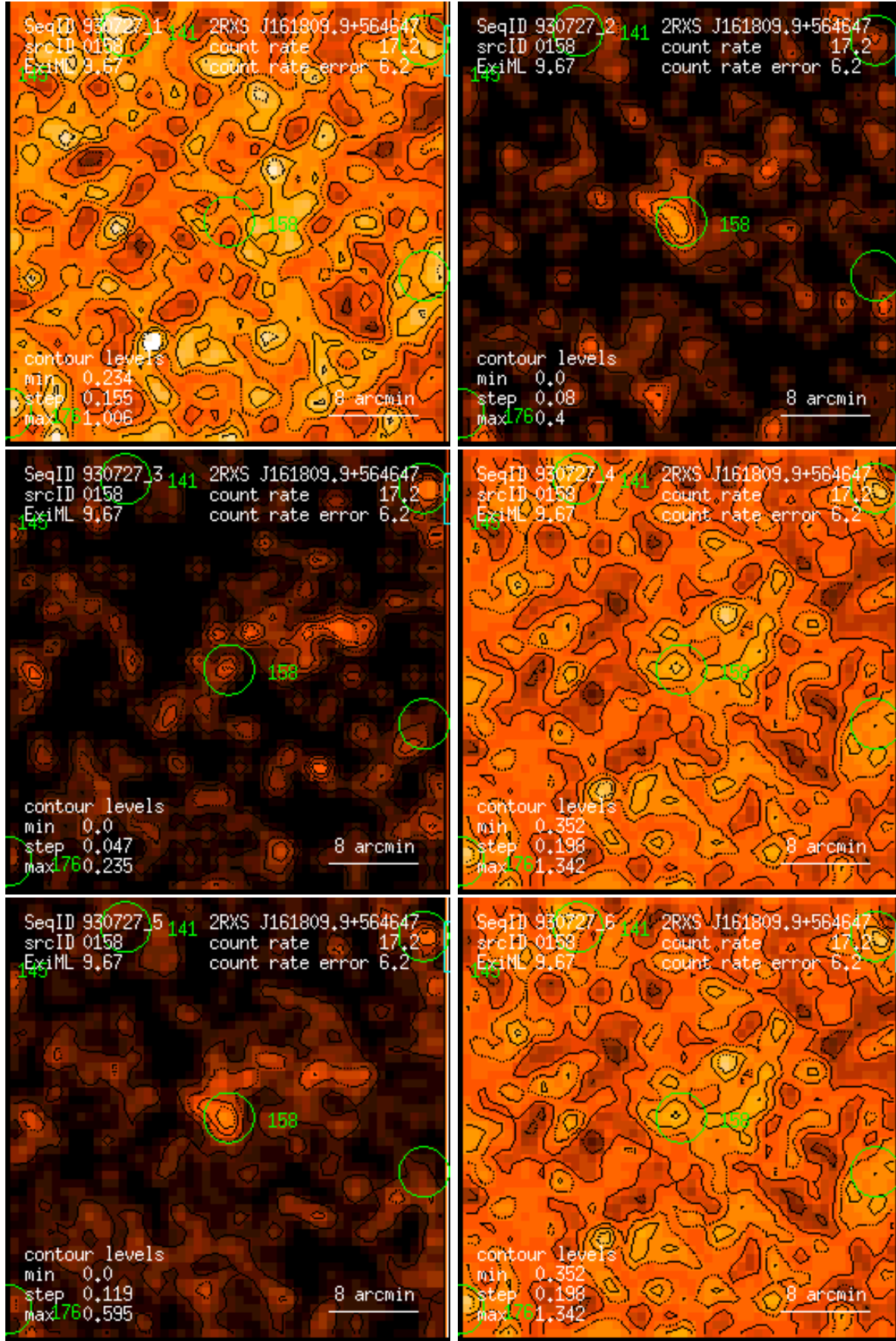
Figure 158: RASS 930727: detection 0158: band rate images, Gaussian filter: (1) PSPC channels 11 – 41, (2) 52 – 90, (3) 91 – 201, (4) 11 – 235, (5) 52 – 201, (6) 11 – 201. Broad band rates in counts/ks. Band rate contour levels in counts/ks/arcmin 2 .
