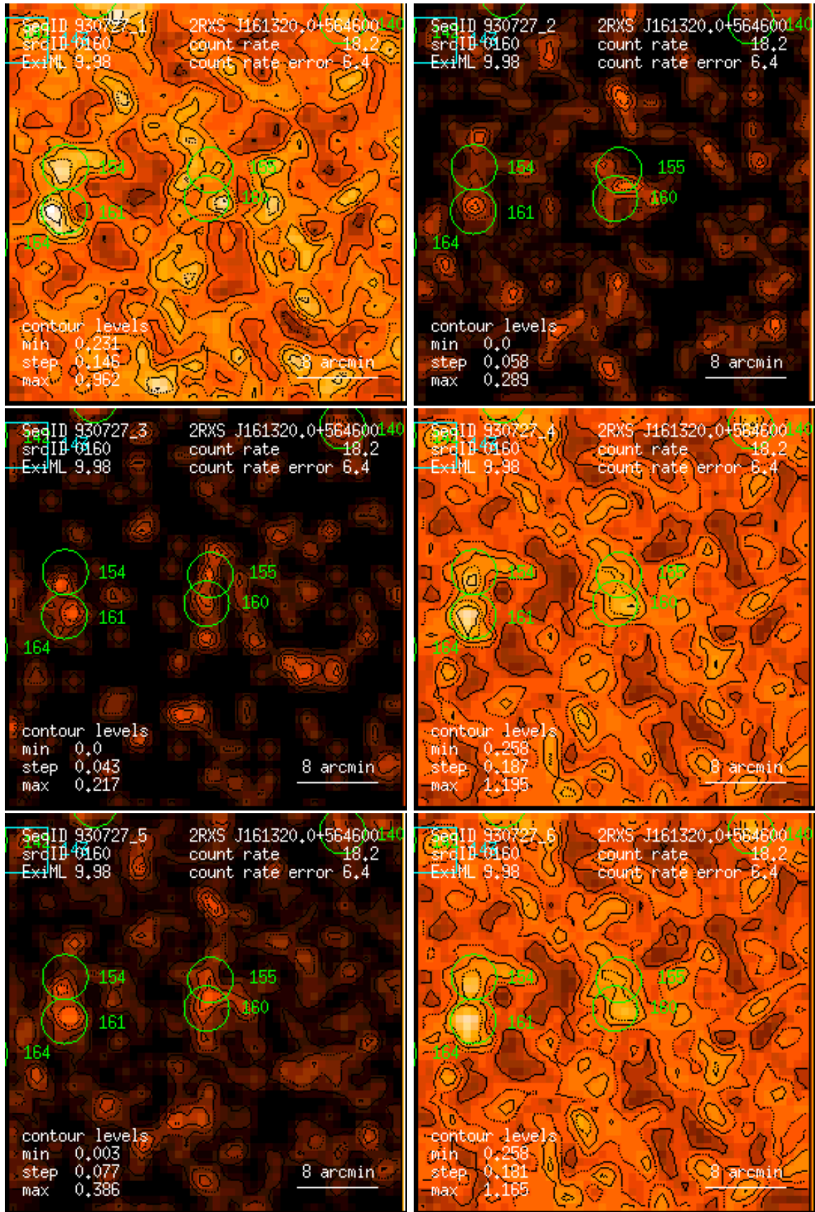
Figure 160: RASS 930727: detection 0160: band rate images, Gaussian filter: (1) PSPC channels 11 – 41, (2) 52 – 90, (3) 91 – 201, (4) 11 – 235, (5) 52 – 201, (6) 11 – 201. Broad band rates in counts/ks. Band rate contour levels in counts/ks/arcmin 2 .
