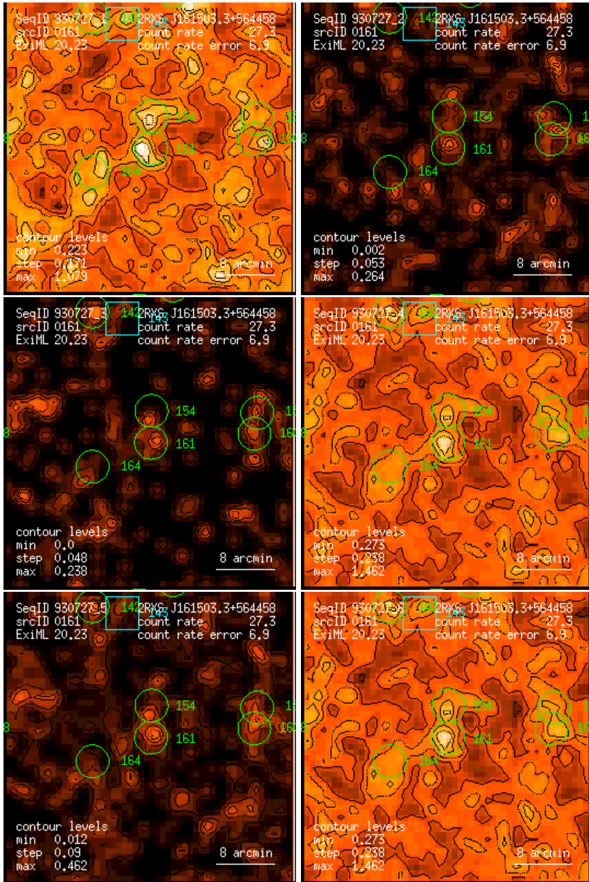
Figure 161: RASS 930727: detection 0161: band rate images, Gaussian filter: (1) PSPC channels 11 – 41, (2) 52 – 90, (3) 91 – 201, (4) 11 – 235, (5) 52 – 201, (6) 11 – 201. Broad band rates in counts/ks. Band rate contour levels in counts/ks/arcmin 2 .
