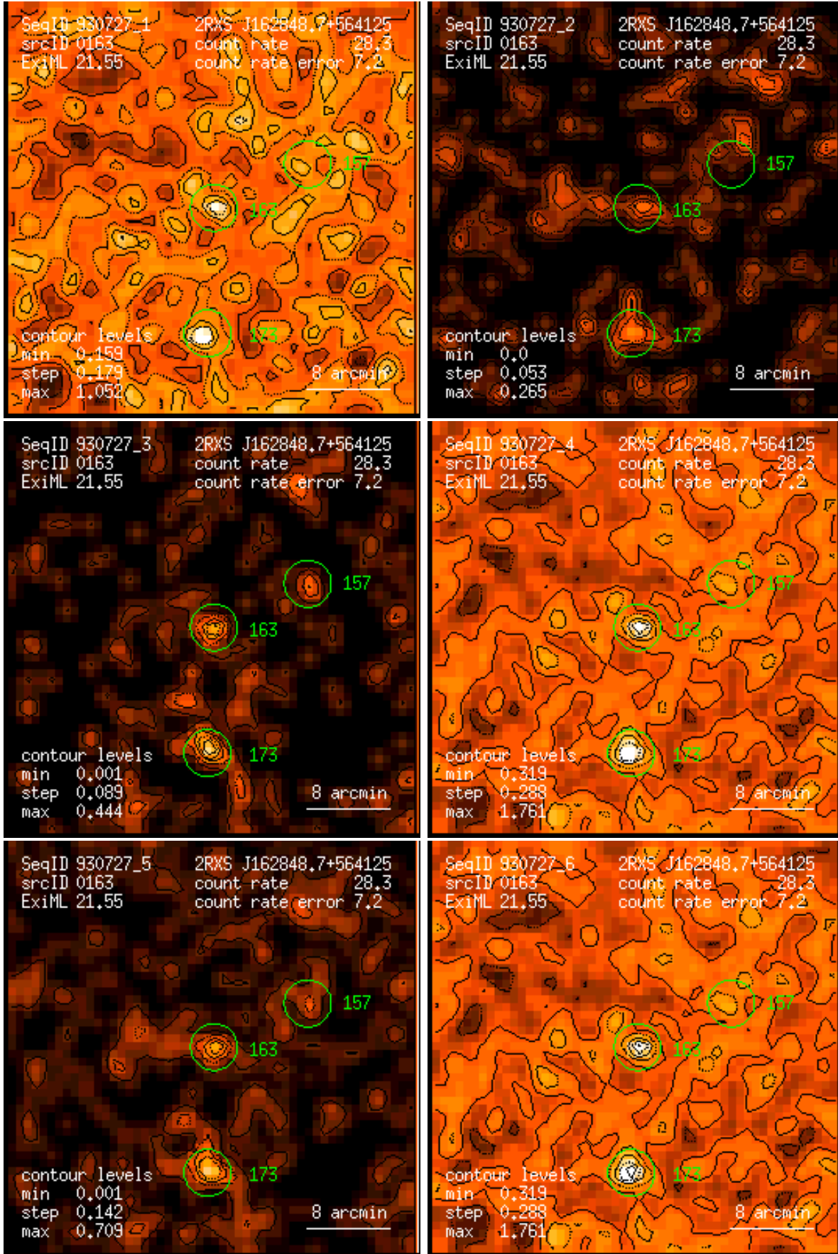
Figure 163: RASS 930727: detection 0163: band rate images, Gaussian filter: (1) PSPC channels 11 – 41, (2) 52 – 90, (3) 91 – 201, (4) 11 – 235, (5) 52 – 201, (6) 11 – 201. Broad band rates in counts/ks. Band rate contour levels in counts/ks/arcmin 2 .
