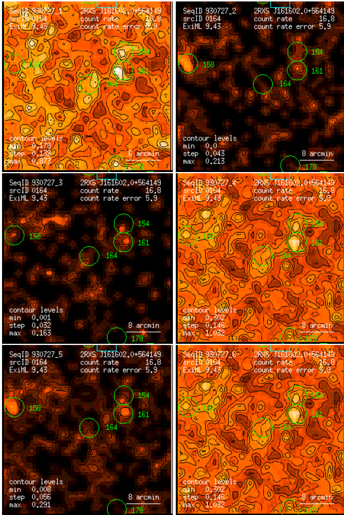
Figure 164: RASS 930727: detection 0164: band rate images, Gaussian filter: (1) PSPC channels 11 – 41, (2) 52 – 90, (3) 91 – 201, (4) 11 – 235, (5) 52 – 201, (6) 11 – 201. Broad band rates in counts/ks. Band rate contour levels in counts/ks/arcmin 2 .
