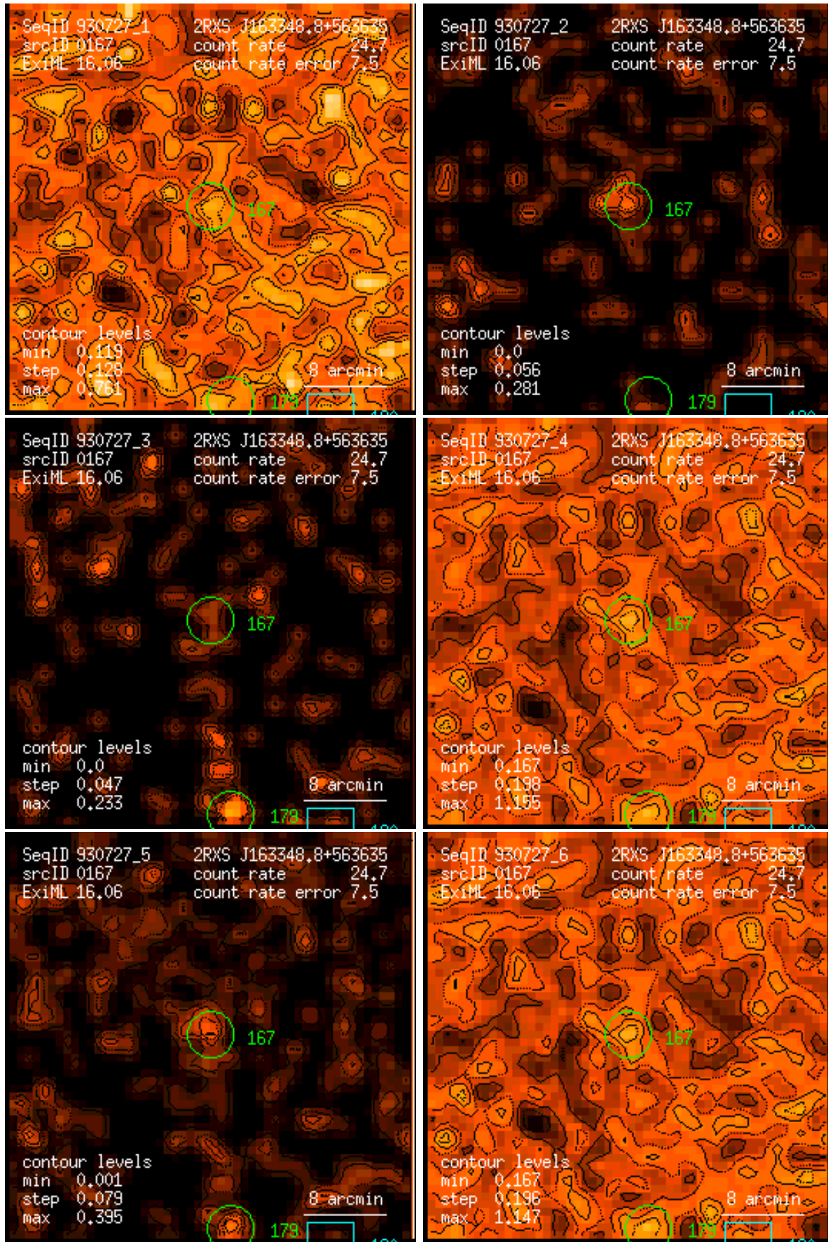
Figure 167: RASS 930727: detection 0167: band rate images, Gaussian filter: (1) PSPC channels 11 – 41, (2) 52 – 90, (3) 91 – 201, (4) 11 – 235, (5) 52 – 201, (6) 11 – 201. Broad band rates in counts/ks. Band rate contour levels in counts/ks/arcmin 2 .
