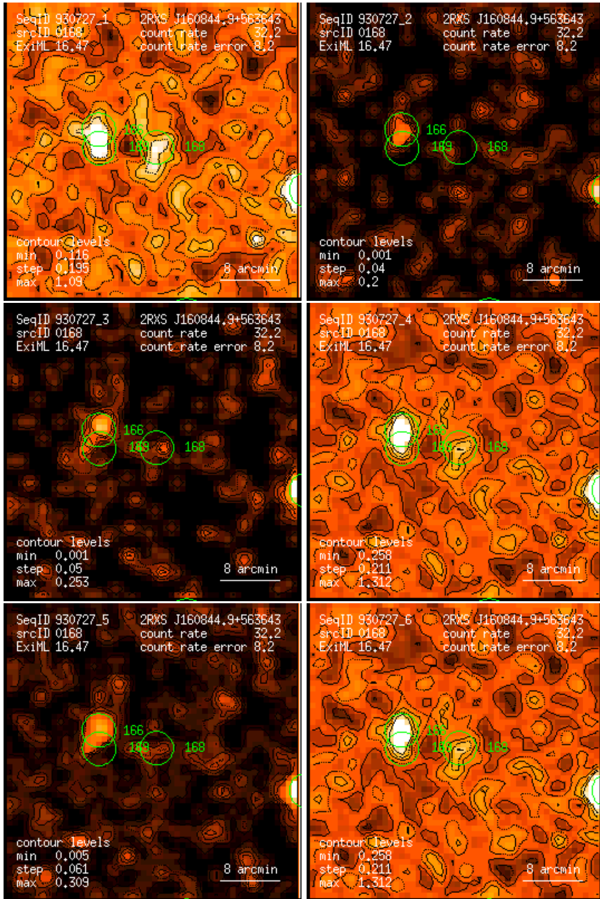
Figure 168: RASS 930727: detection 0168: band rate images, Gaussian filter: (1) PSPC channels 11 – 41, (2) 52 – 90, (3) 91 – 201, (4) 11 – 235, (5) 52 – 201, (6) 11 – 201. Broad band rates in counts/ks. Band rate contour levels in counts/ks/arcmin 2 .
