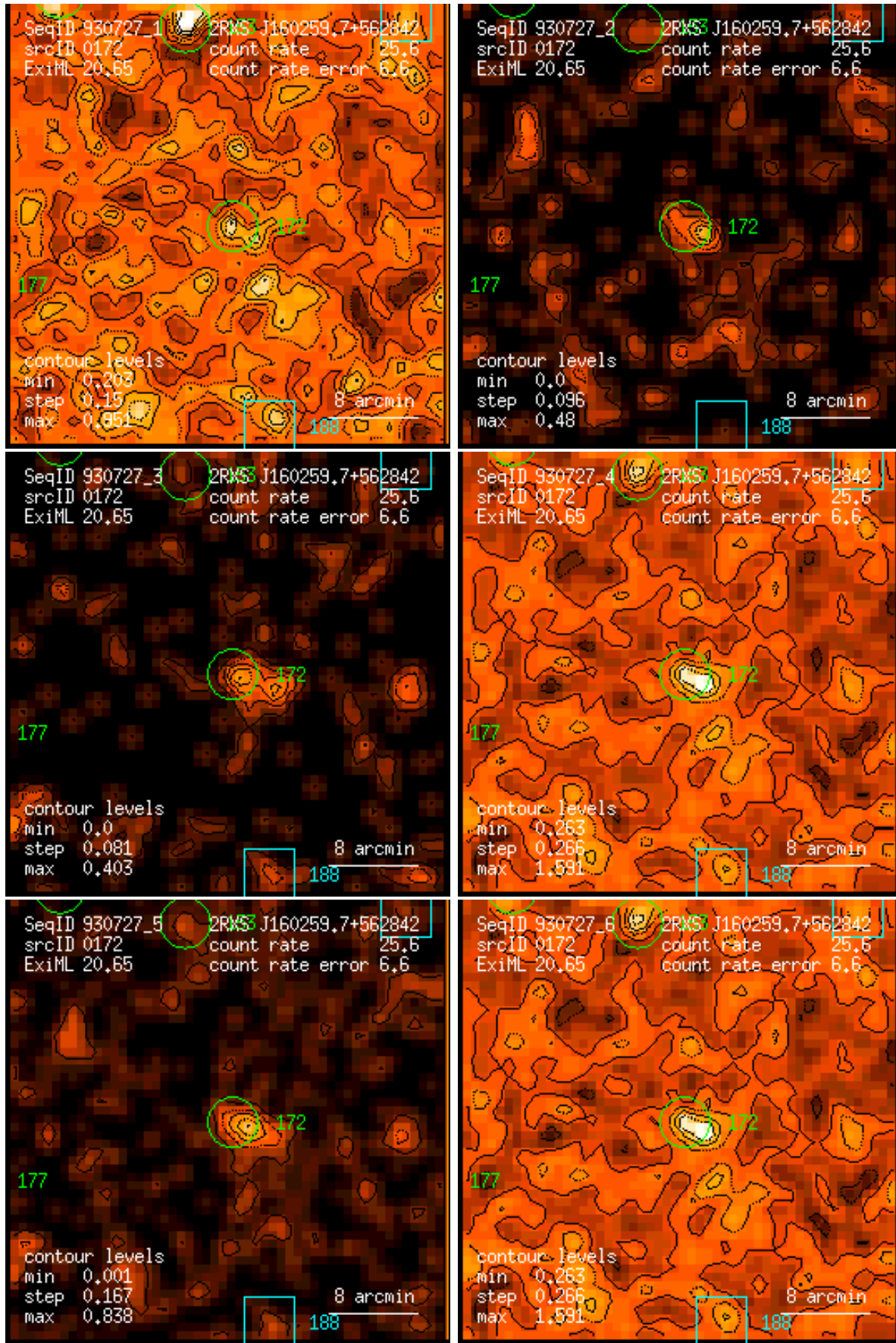
Figure 172: RASS 930727: detection 0172: band rate images, Gaussian filter: (1) PSPC channels 11 – 41, (2) 52 – 90, (3) 91 – 201, (4) 11 – 235, (5) 52 – 201, (6) 11 – 201. Broad band rates in counts/ks. Band rate contour levels in counts/ks/arcmin 2 .
