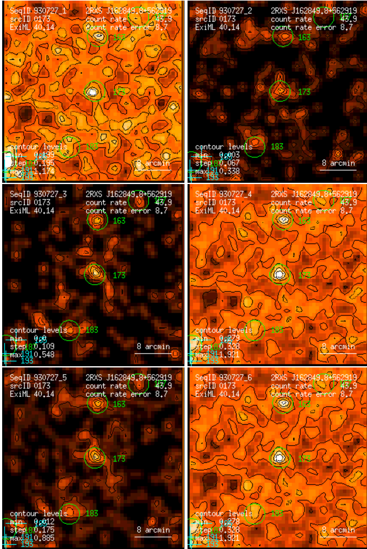
Figure 173: RASS 930727: detection 0173: band rate images, Gaussian filter: (1) PSPC channels 11 – 41, (2) 52 – 90, (3) 91 – 201, (4) 11 – 235, (5) 52 – 201, (6) 11 – 201. Broad band rates in counts/ks. Band rate contour levels in counts/ks/arcmin 2 .
