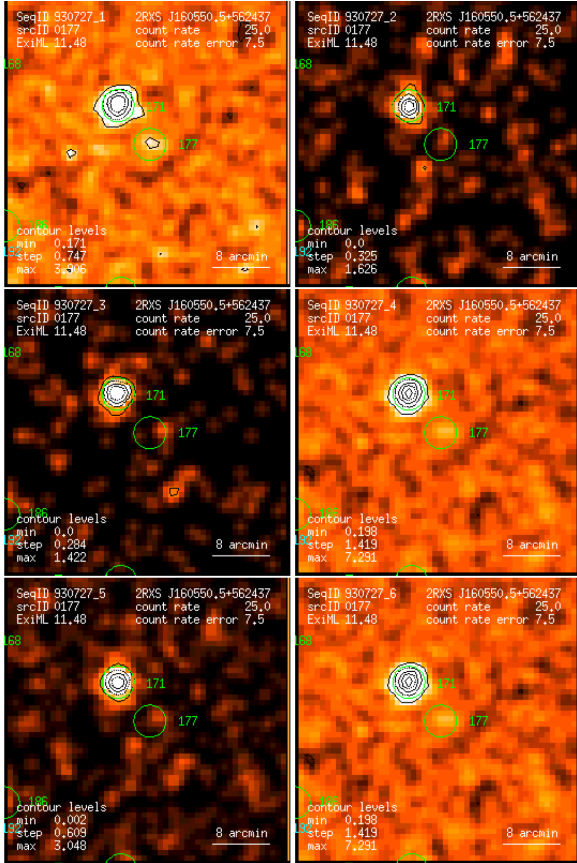
Figure 177: RASS 930727: detection 0177: band rate images, Gaussian filter: (1) PSPC channels 11 – 41, (2) 52 – 90, (3) 91 – 201, (4) 11 – 235, (5) 52 – 201, (6) 11 – 201. Broad band rates in counts/ks. Band rate contour levels in counts/ks/arcmin 2 .
