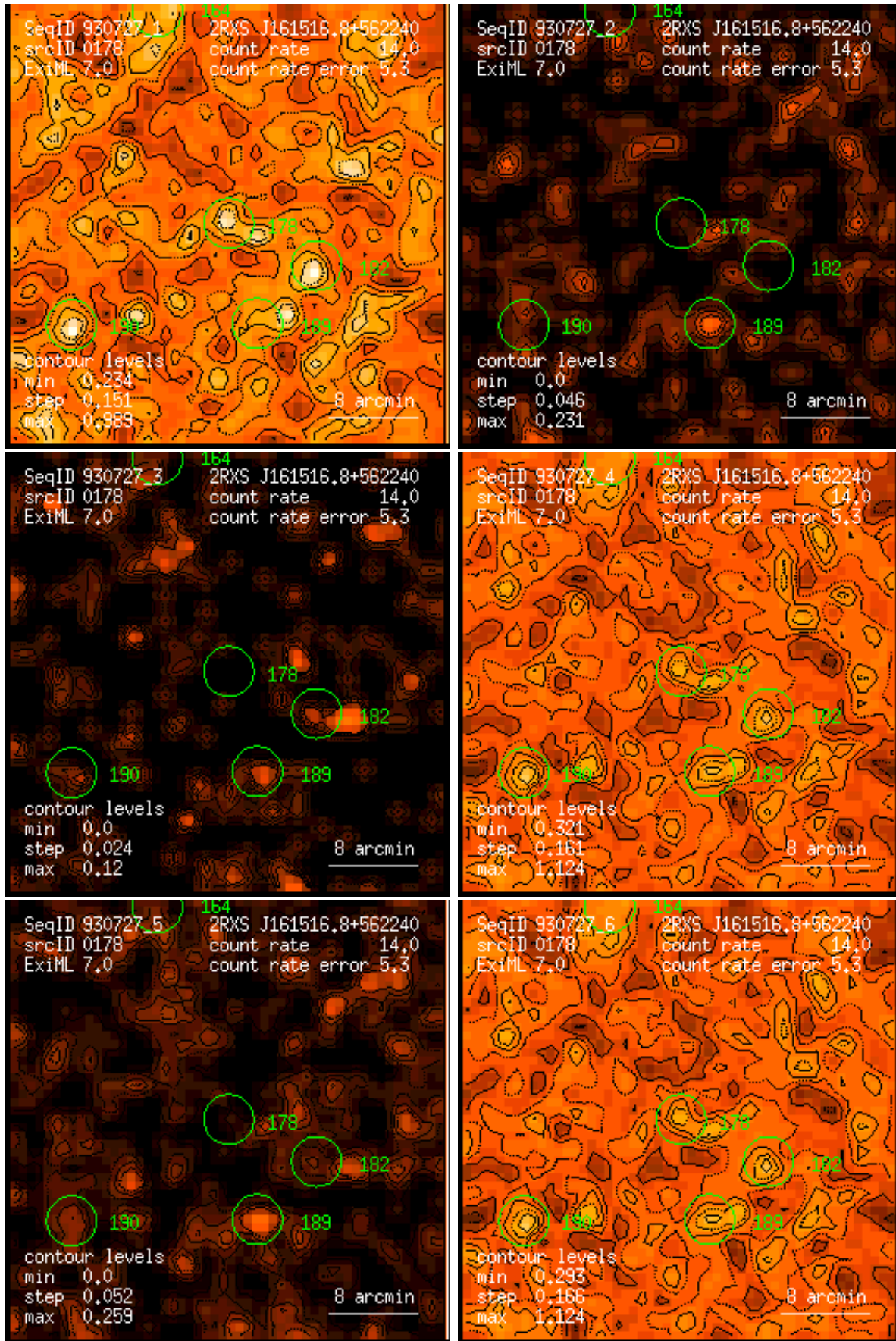
Figure 178: RASS 930727: detection 0178: band rate images, Gaussian filter: (1) PSPC channels 11 – 41, (2) 52 – 90, (3) 91 – 201, (4) 11 – 235, (5) 52 – 201, (6) 11 – 201. Broad band rates in counts/ks. Band rate contour levels in counts/ks/arcmin 2 .
