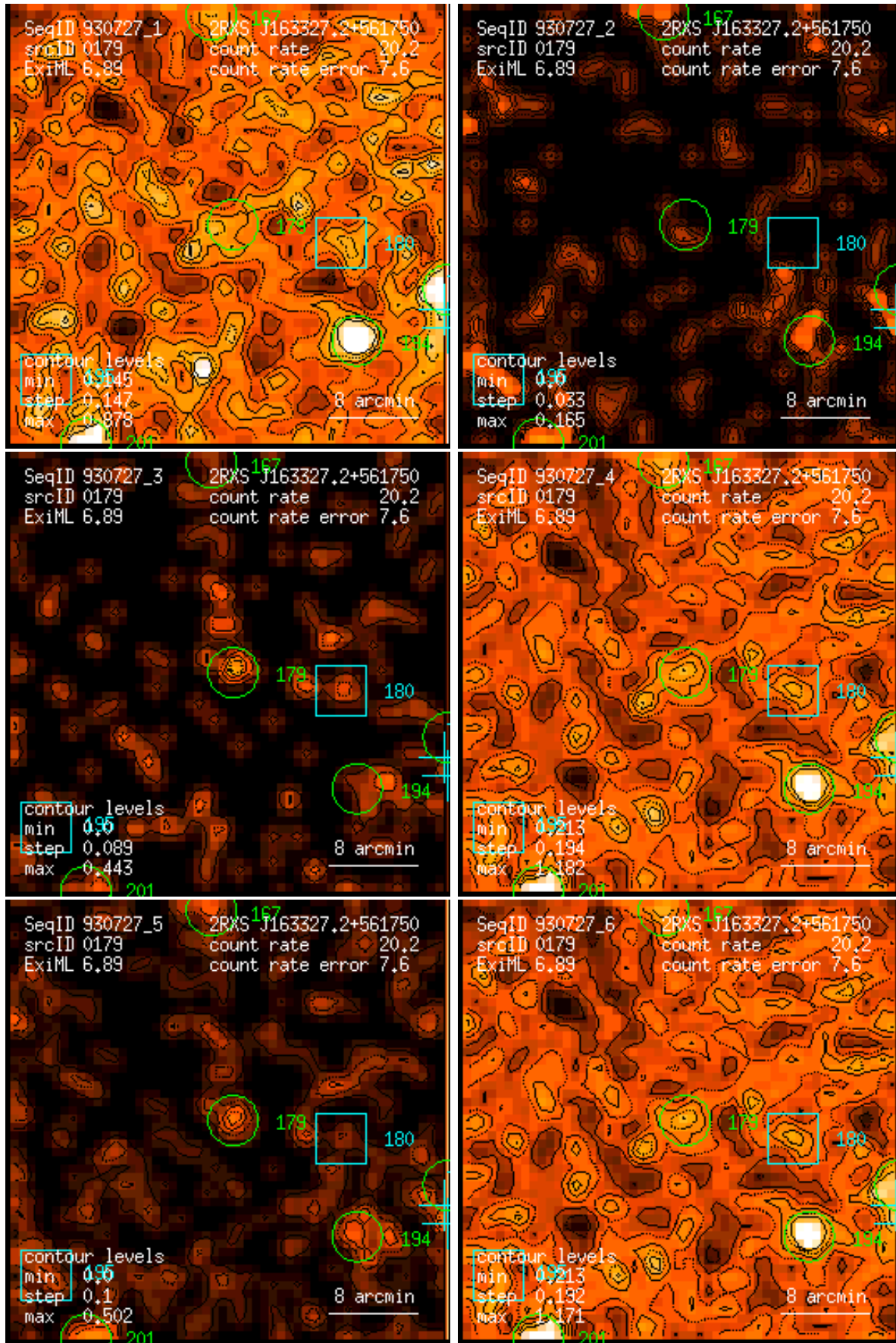
Figure 179: RASS 930727: detection 0179: band rate images, Gaussian filter: (1) PSPC channels 11 – 41, (2) 52 – 90, (3) 91 – 201, (4) 11 – 235, (5) 52 – 201, (6) 11 – 201. Broad band rates in counts/ks. Band rate contour levels in counts/ks/arcmin 2 .
