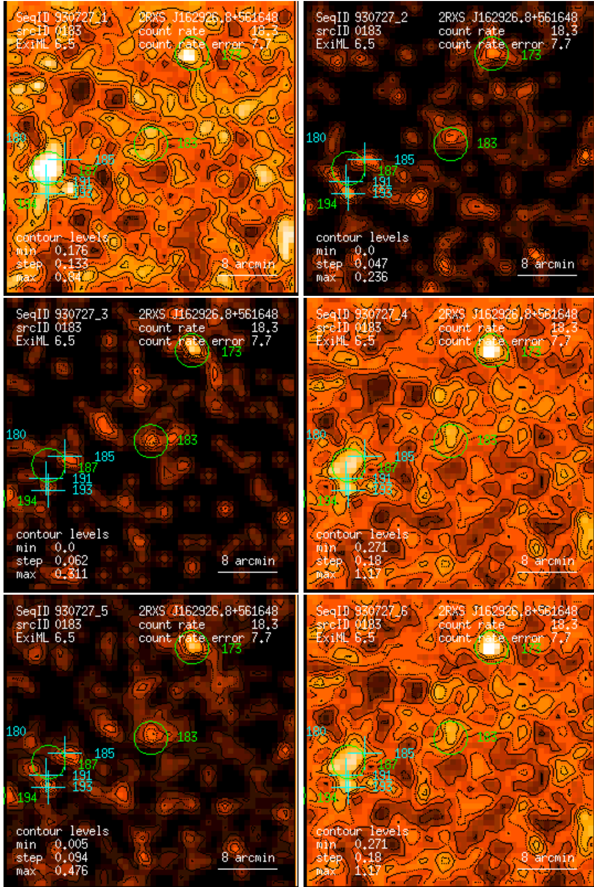
Figure 183: RASS 930727: detection 0183: band rate images, Gaussian filter: (1) PSPC channels 11 – 41, (2) 52 – 90, (3) 91 – 201, (4) 11 – 235, (5) 52 – 201, (6) 11 – 201. Broad band rates in counts/ks. Band rate contour levels in counts/ks/arcmin 2 .
