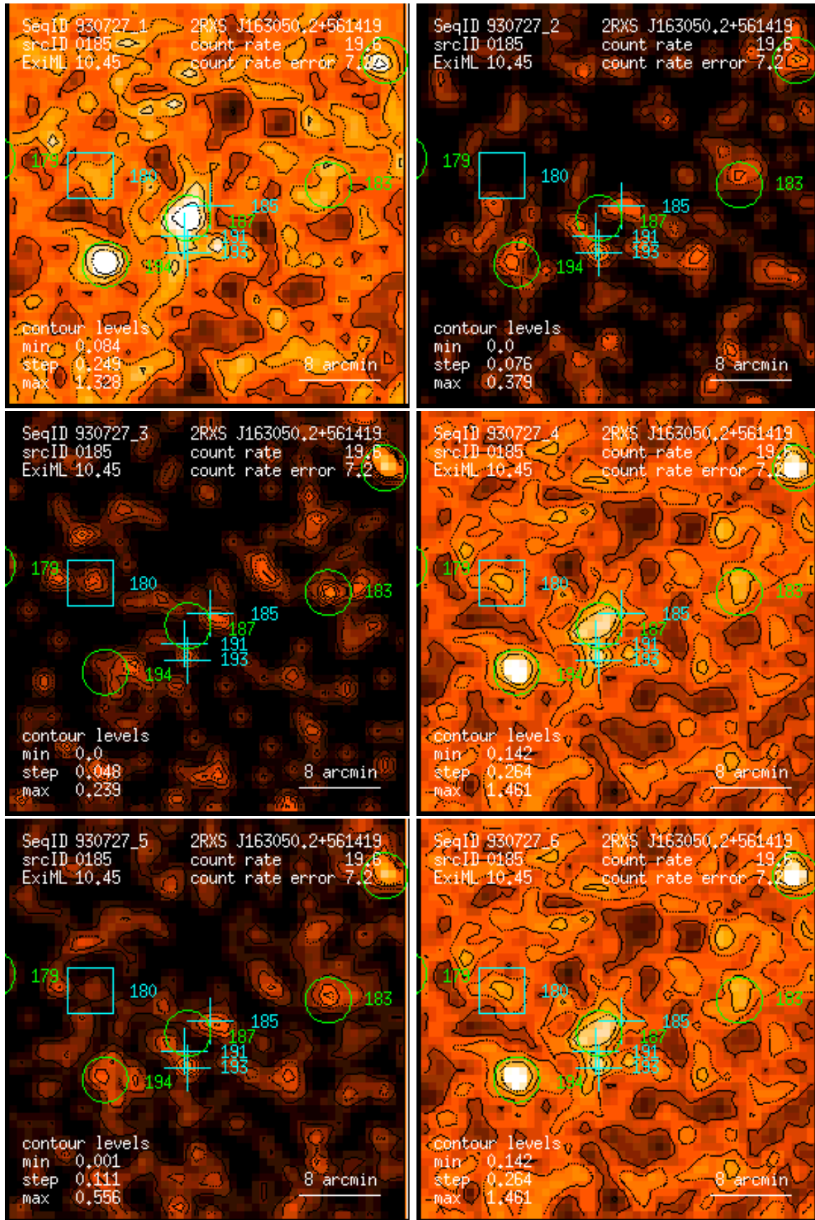
Figure 185: RASS 930727: detection 0185: band rate images, Gaussian filter: (1) PSPC channels 11 – 41, (2) 52 – 90, (3) 91 – 201, (4) 11 – 235, (5) 52 – 201, (6) 11 – 201. Broad band rates in counts/ks. Band rate contour levels in counts/ks/arcmin 2 .
