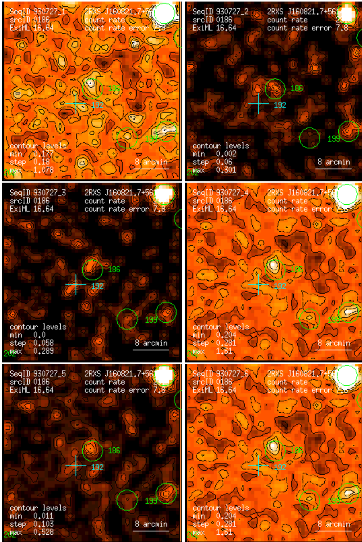
Figure 186: RASS 930727: detection 0186: band rate images, Gaussian filter: (1) PSPC channels 11 – 41, (2) 52 – 90, (3) 91 – 201, (4) 11 – 235, (5) 52 – 201, (6) 11 – 201. Broad band rates in counts/ks. Band rate contour levels in counts/ks/arcmin 2 .
