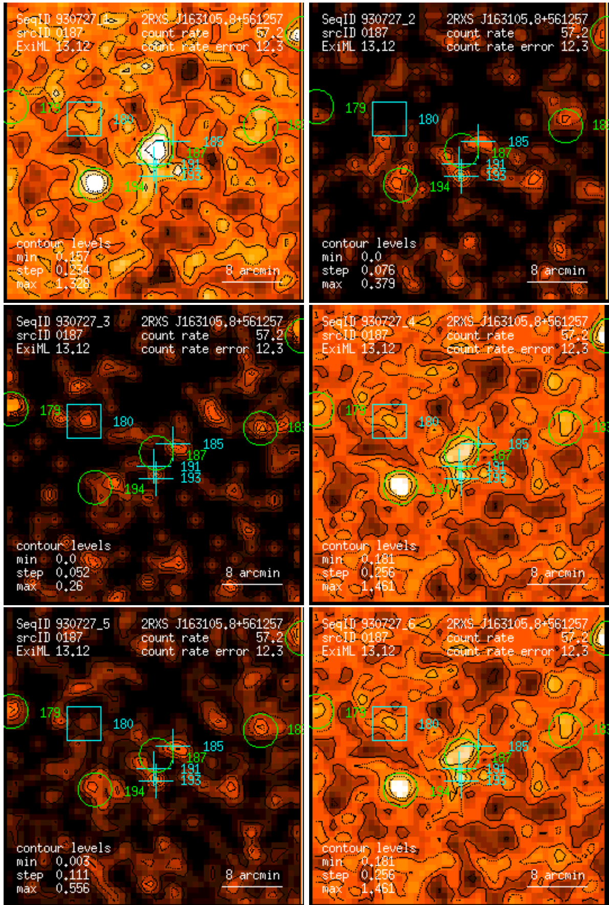
Figure 187: RASS 930727: detection 0187: band rate images, Gaussian filter: (1) PSPC channels 11 – 41, (2) 52 – 90, (3) 91 – 201, (4) 11 – 235, (5) 52 – 201, (6) 11 – 201. Broad band rates in counts/ks. Band rate contour levels in counts/ks/arcmin 2 .
