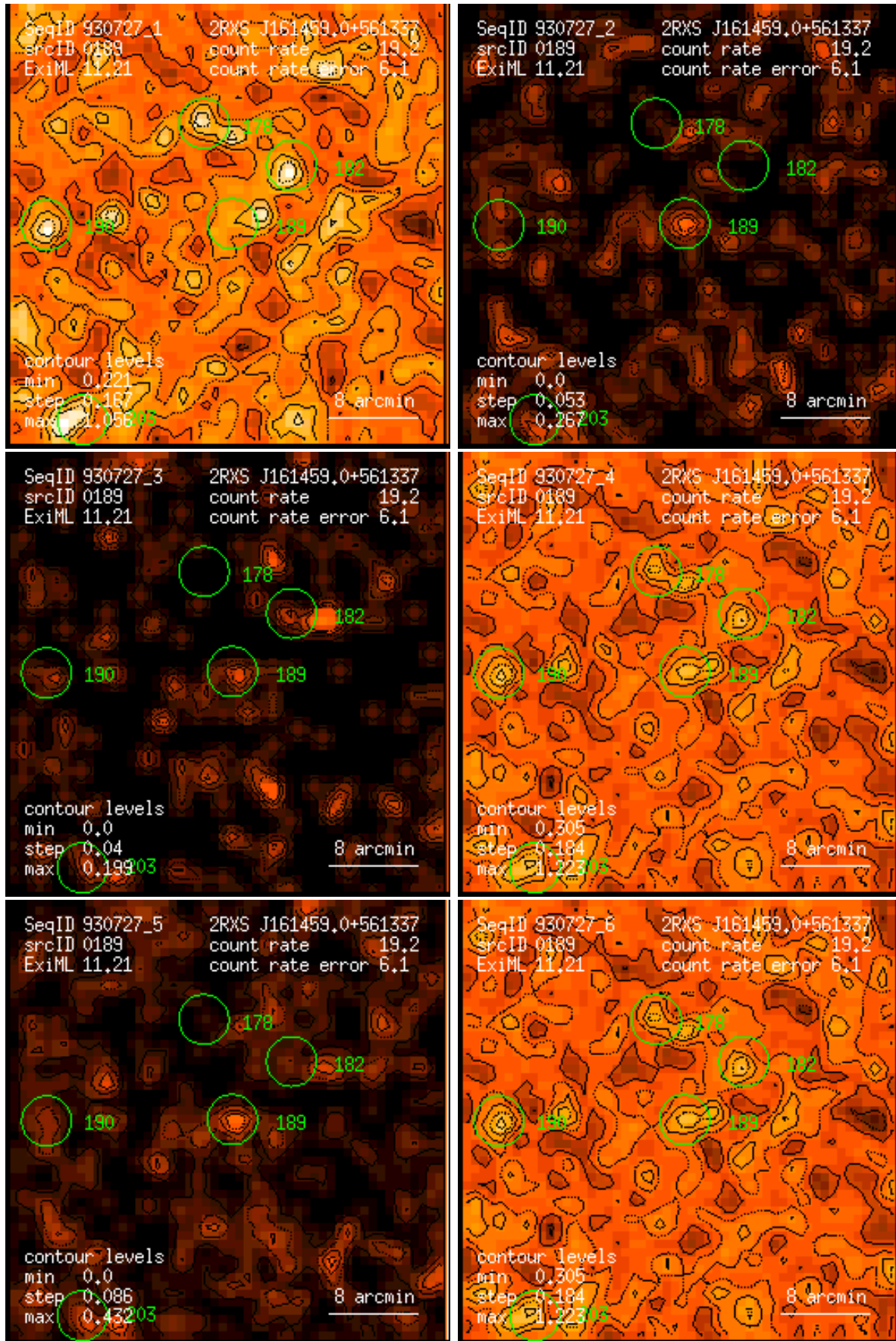
Figure 189: RASS 930727: detection 0189: band rate images, Gaussian filter: (1) PSPC channels 11 – 41, (2) 52 – 90, (3) 91 – 201, (4) 11 – 235, (5) 52 – 201, (6) 11 – 201. Broad band rates in counts/ks. Band rate contour levels in counts/ks/arcmin 2 .
