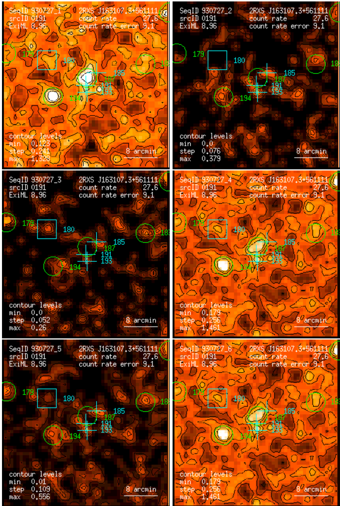
Figure 191: RASS 930727: detection 0191: band rate images, Gaussian filter: (1) PSPC channels 11 – 41, (2) 52 – 90, (3) 91 – 201, (4) 11 – 235, (5) 52 – 201, (6) 11 – 201. Broad band rates in counts/ks. Band rate contour levels in counts/ks/arcmin 2 .
