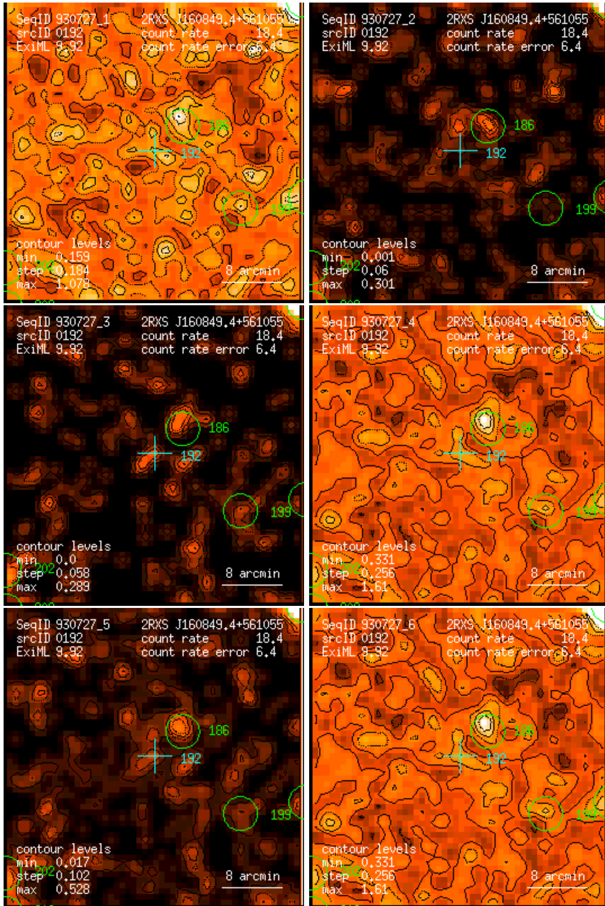
Figure 192: RASS 930727: detection 0192: band rate images, Gaussian filter: (1) PSPC channels 11 – 41, (2) 52 – 90, (3) 91 – 201, (4) 11 – 235, (5) 52 – 201, (6) 11 – 201. Broad band rates in counts/ks. Band rate contour levels in counts/ks/arcmin 2 .
