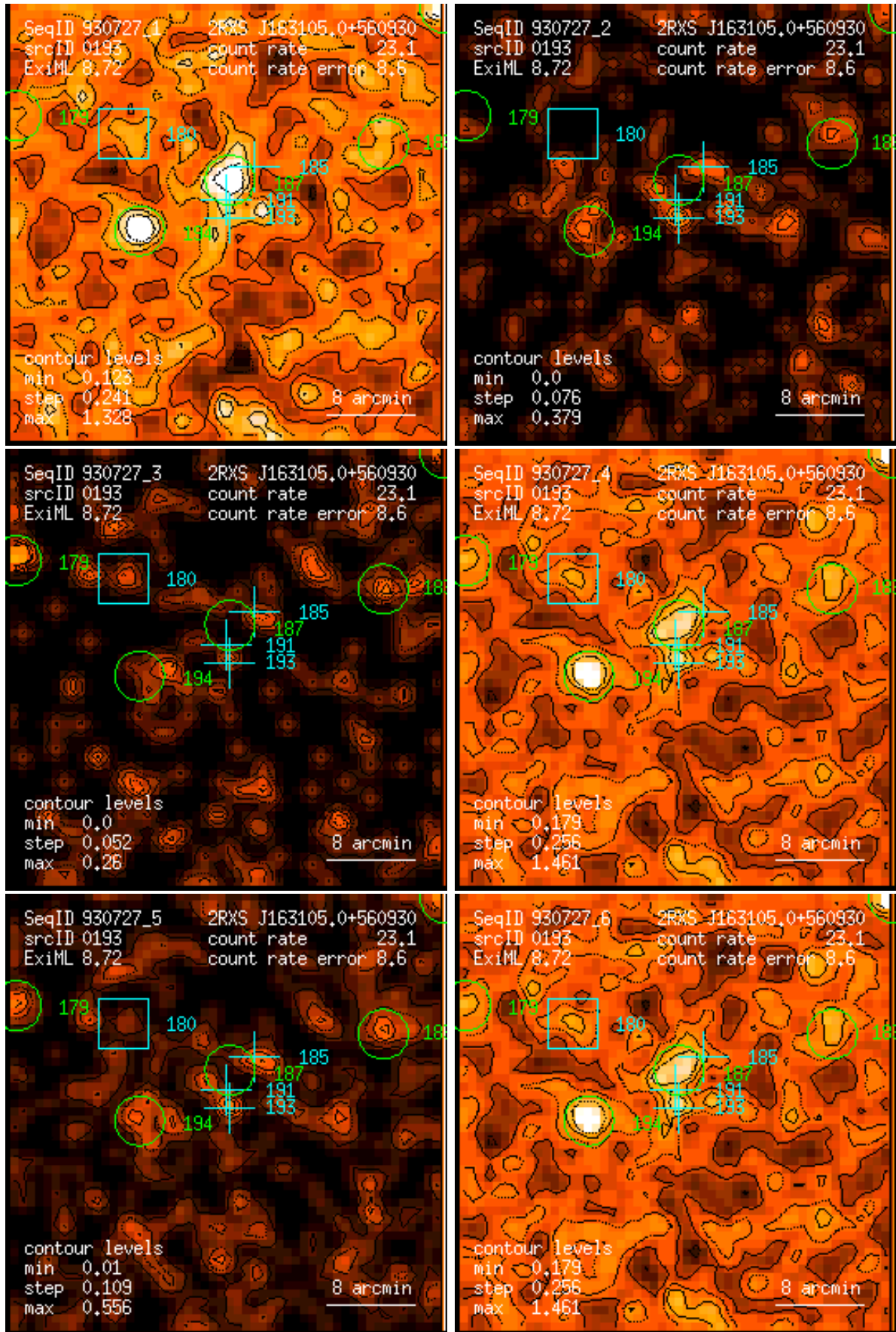
Figure 193: RASS 930727: detection 0193: band rate images, Gaussian filter: (1) PSPC channels 11 – 41, (2) 52 – 90, (3) 91 – 201, (4) 11 – 235, (5) 52 – 201, (6) 11 – 201. Broad band rates in counts/ks. Band rate contour levels in counts/ks/arcmin 2 .
