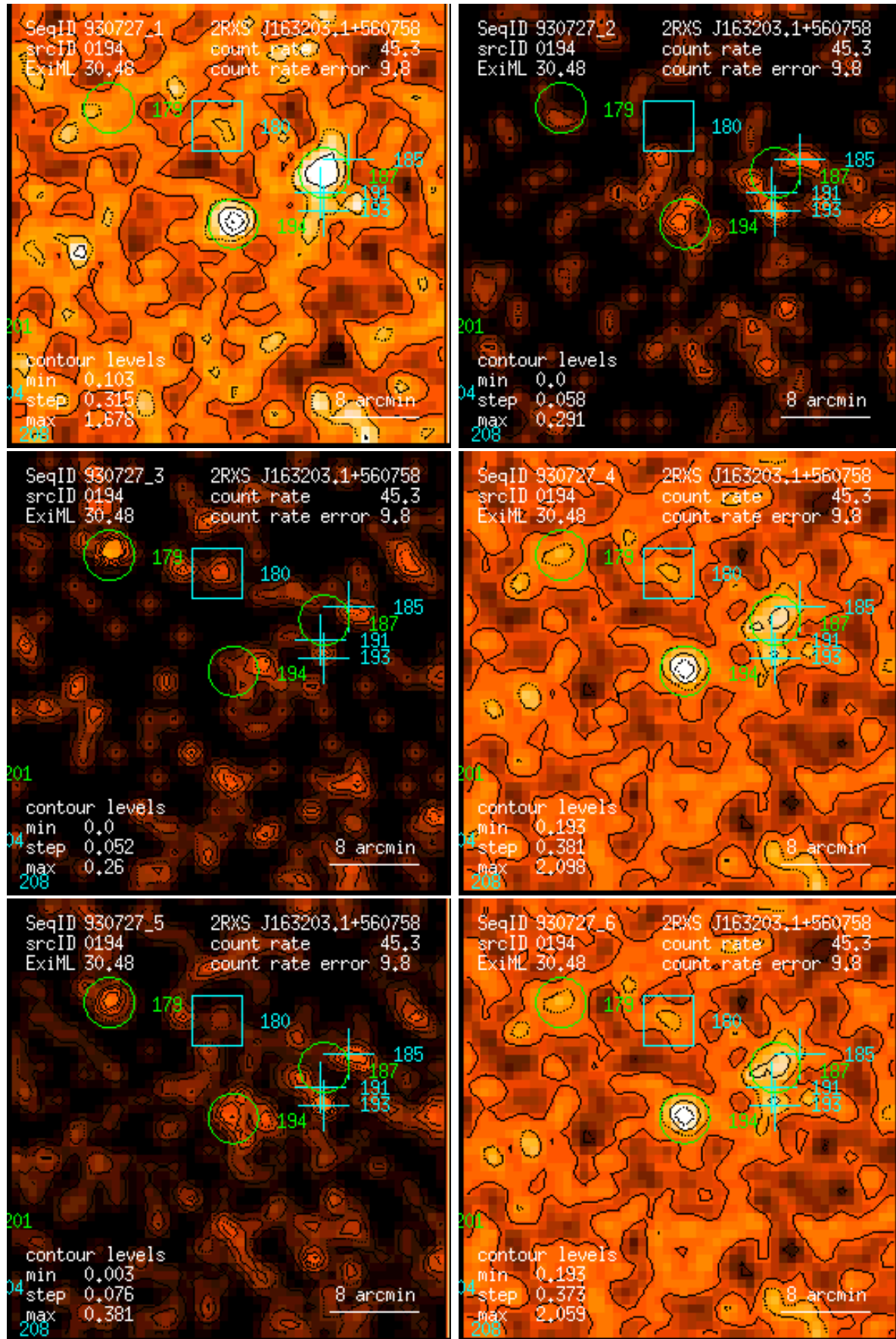
Figure 194: RASS 930727: detection 0194: band rate images, Gaussian filter: (1) PSPC channels 11 – 41, (2) 52 – 90, (3) 91 – 201, (4) 11 – 235, (5) 52 – 201, (6) 11 – 201. Broad band rates in counts/ks. Band rate contour levels in counts/ks/arcmin 2 .
