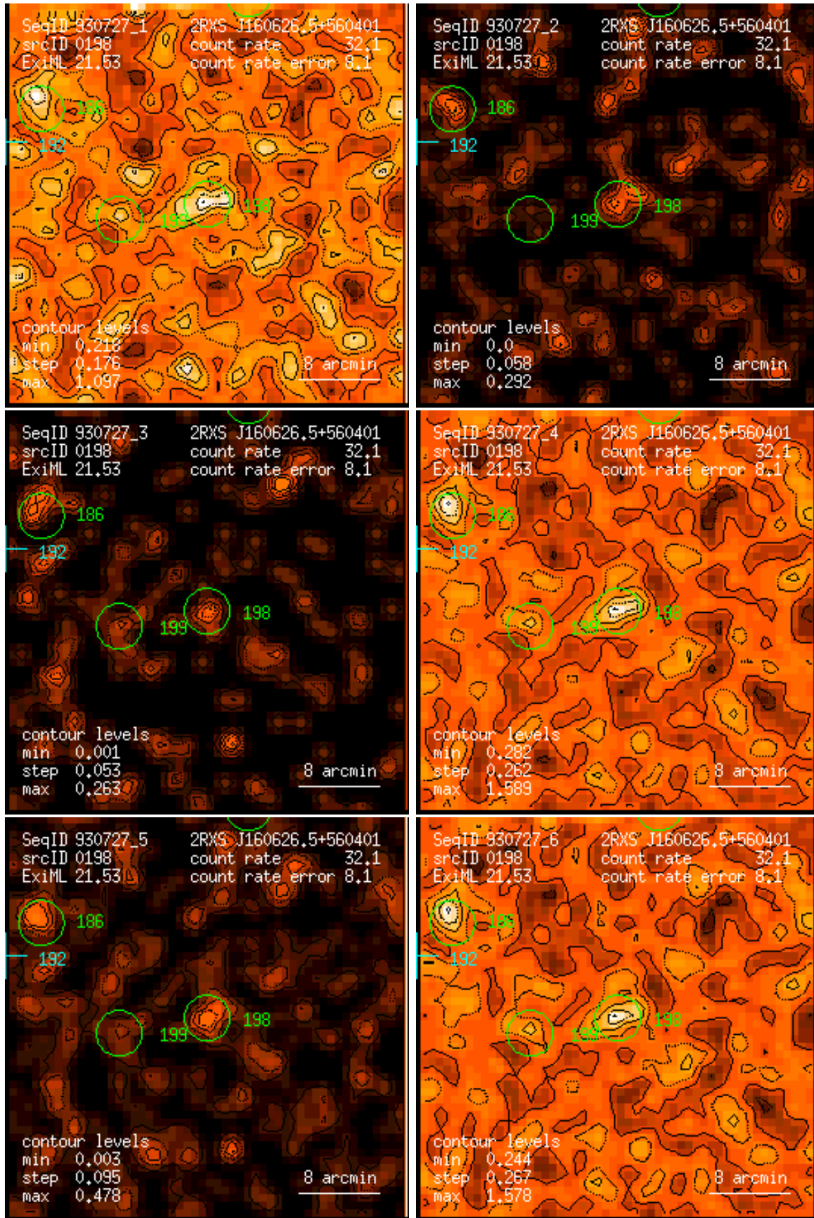
Figure 198: RASS 930727: detection 0198: band rate images, Gaussian filter: (1) PSPC channels 11 – 41, (2) 52 – 90, (3) 91 – 201, (4) 11 – 235, (5) 52 – 201, (6) 11 – 201. Broad band rates in counts/ks. Band rate contour levels in counts/ks/arcmin 2 .
