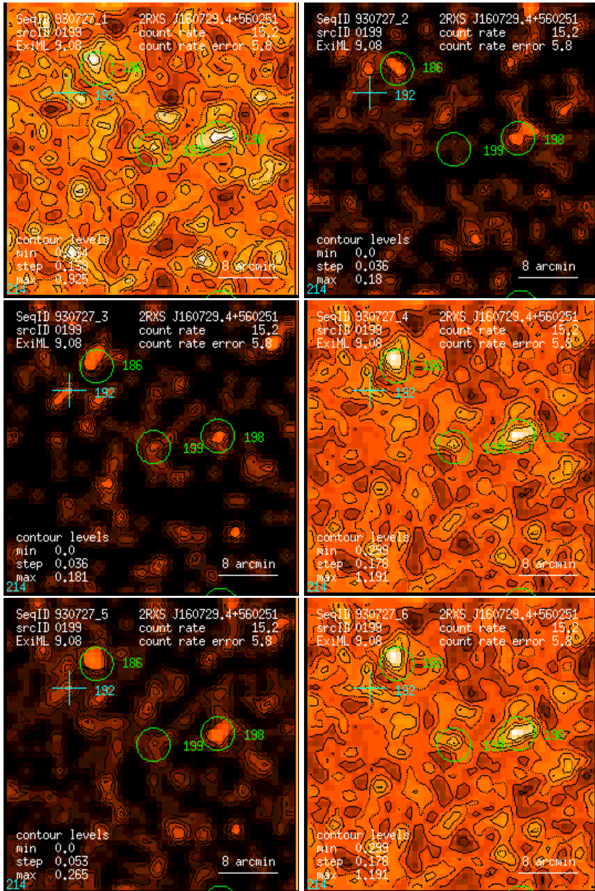
Figure 199: RASS 930727: detection 0199: band rate images, Gaussian filter: (1) PSPC channels 11 – 41, (2) 52 – 90, (3) 91 – 201, (4) 11 – 235, (5) 52 – 201, (6) 11 – 201. Broad band rates in counts/ks. Band rate contour levels in counts/ks/arcmin 2 .
