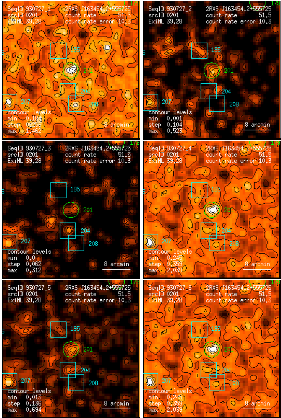
Figure 201: RASS 930727: detection 0201: band rate images, Gaussian filter: (1) PSPC channels 11 – 41, (2) 52 – 90, (3) 91 – 201, (4) 11 – 235, (5) 52 – 201, (6) 11 – 201. Broad band rates in counts/ks. Band rate contour levels in counts/ks/arcmin 2 .
