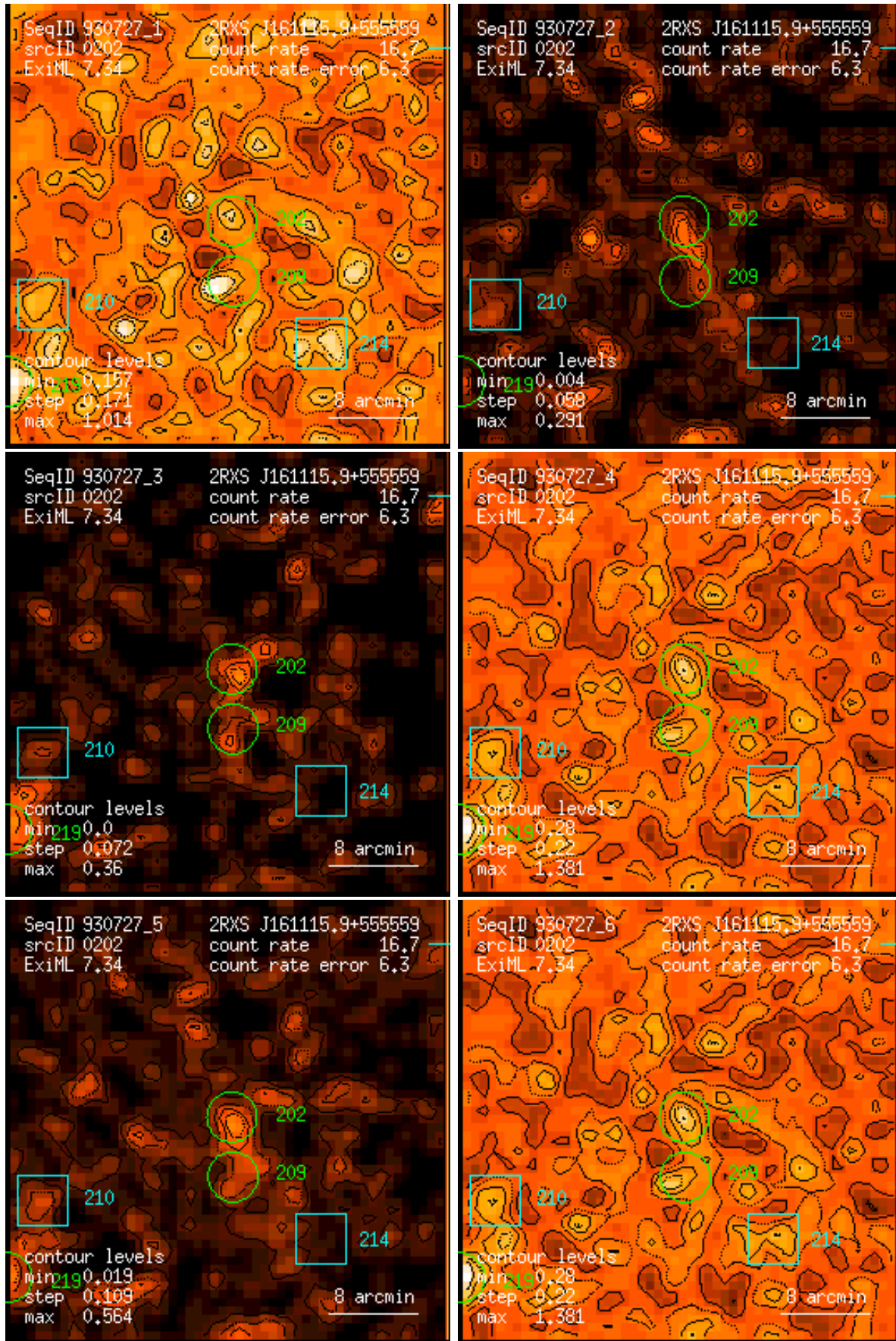
Figure 202: RASS 930727: detection 0202: band rate images, Gaussian filter: (1) PSPC channels 11 – 41, (2) 52 – 90, (3) 91 – 201, (4) 11 – 235, (5) 52 – 201, (6) 11 – 201. Broad band rates in counts/ks. Band rate contour levels in counts/ks/arcmin 2 .
